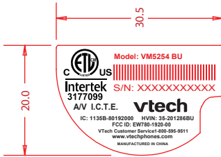
BU LABEL SIZE: 20X30.5mm 50# UL Approved PET
