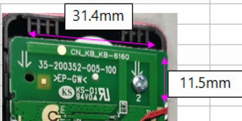
EL52219 HS Antenna Dimensions in mm
