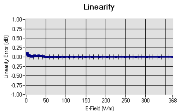
Linearity: \pm 2.40\% ( \pm 0.11 dB)
