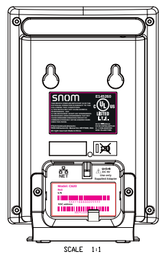
Base station
