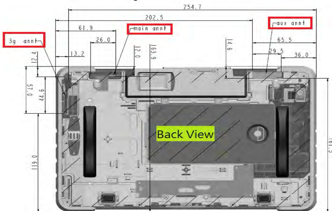
Fig.7 Back view of EUT
