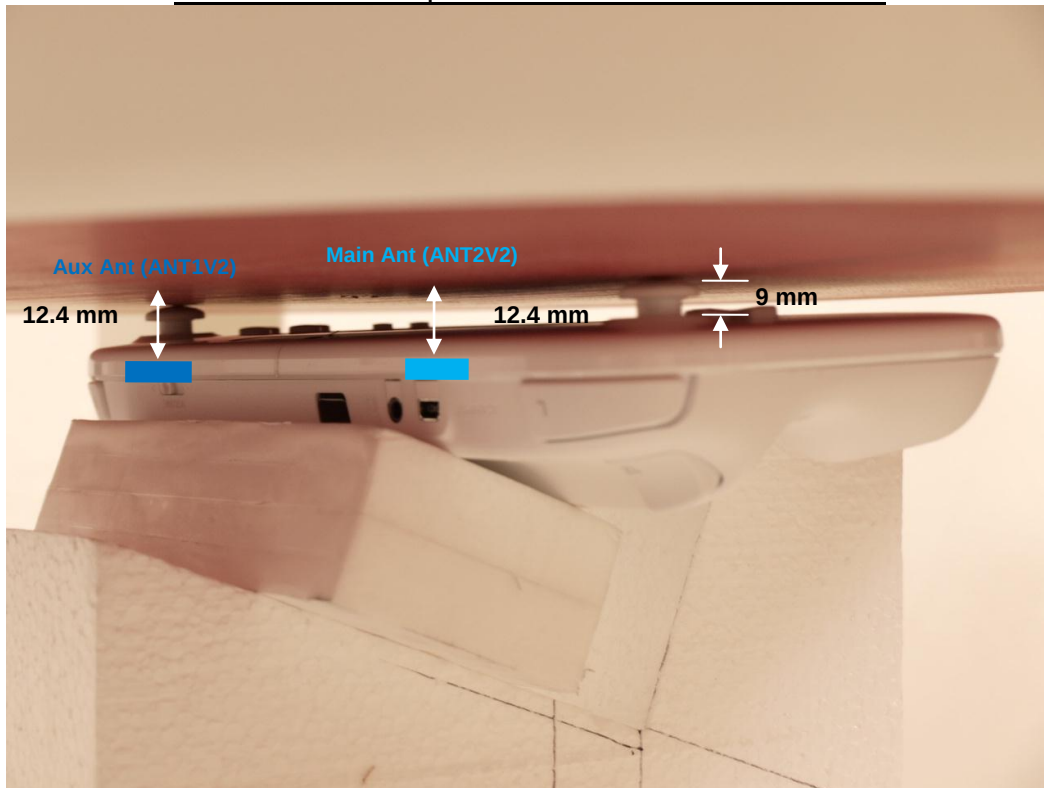
Front w/ 9 mm Separation Distance from Phantom
