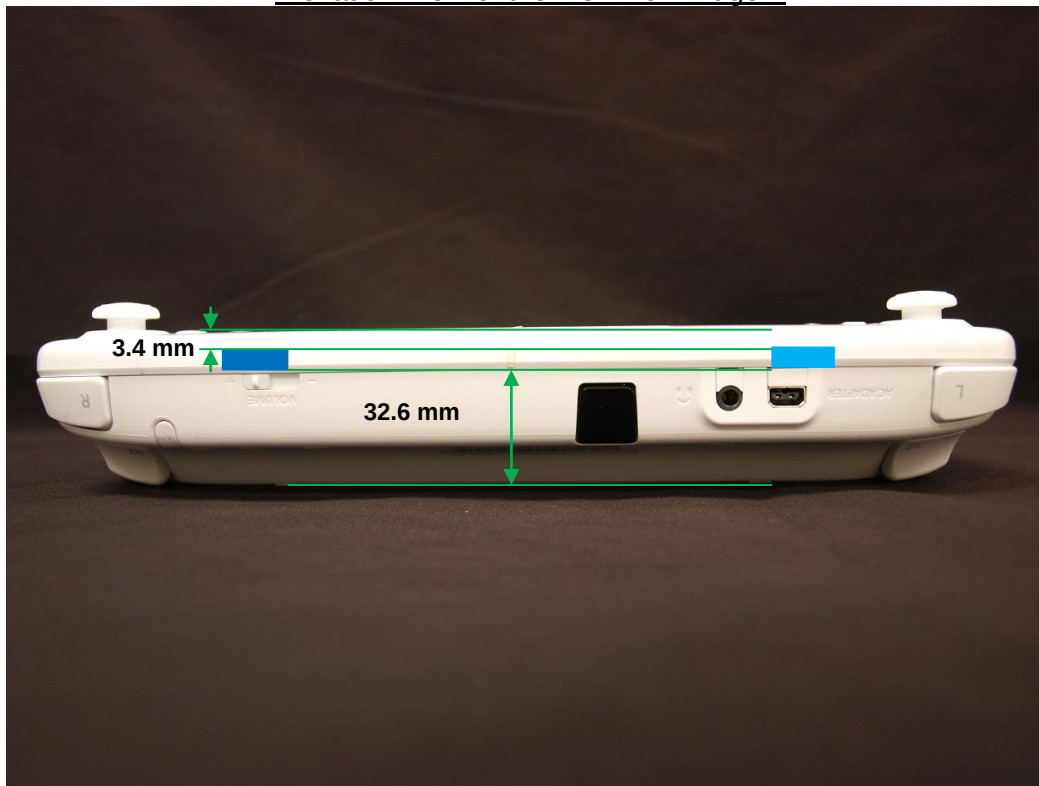
Elevation View of the DUT from Edge 1
