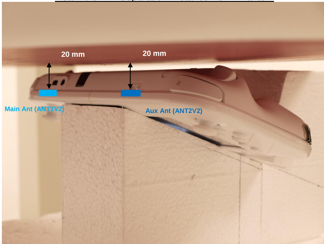
Rear w/ 5 mm Separation Distance from Phantom
