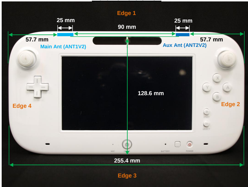
Front View of the DUT
