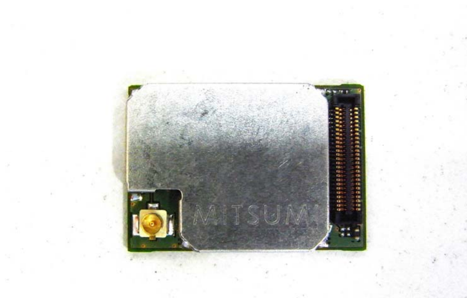
Top view (RF module with shield)
