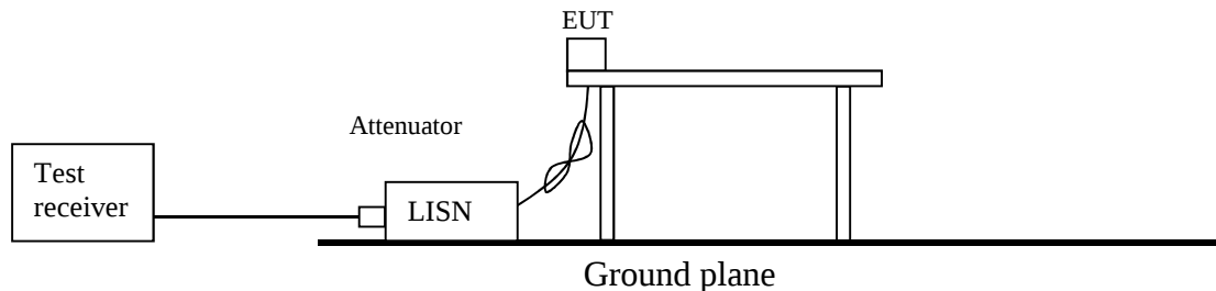
Figure 1: Test Setup
