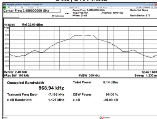
DH5, 2480 MHz
