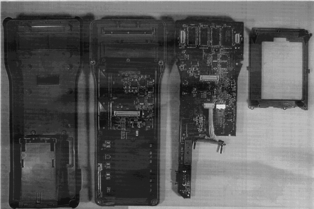
Photo-11: LCD Holder Removed
