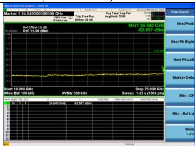
2402MHz(10GHz – 25GHz)
