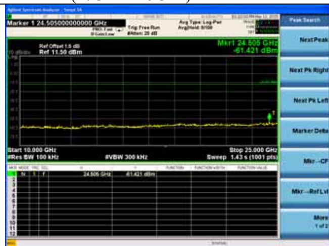
2441MHz(10GHz – 25GHz)
