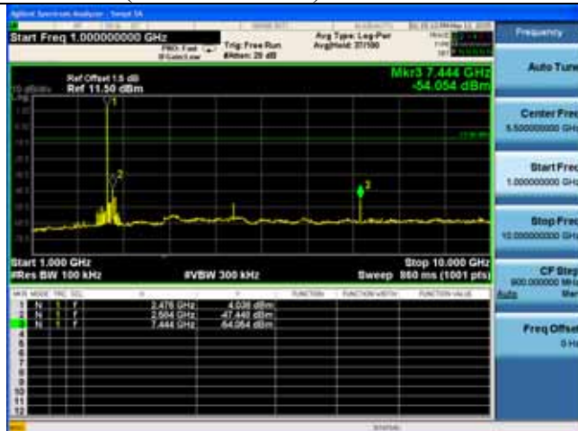
2480MHz(1GHz – 10GHz)
