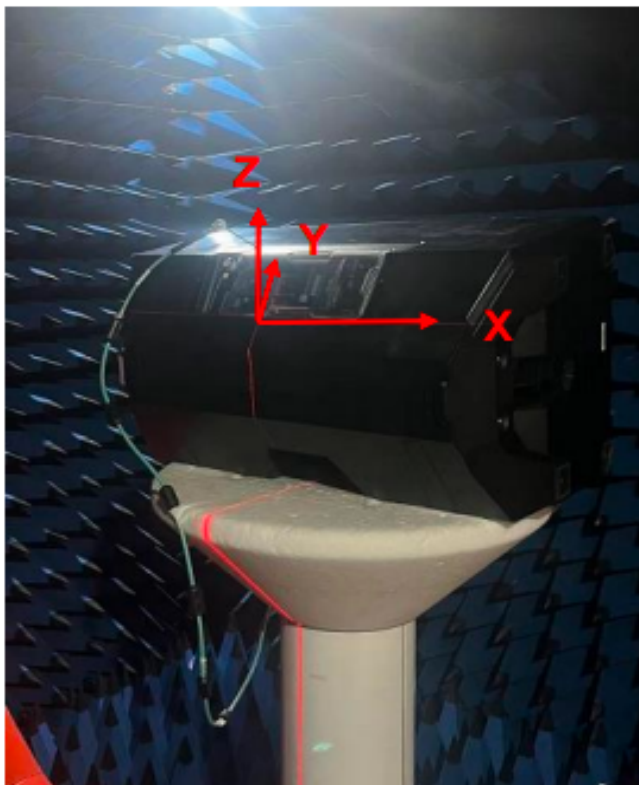
Test Setup
