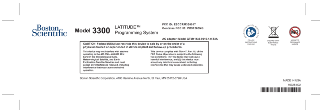
Figure 1 BSC Model 3300 – Back Label Drawing
