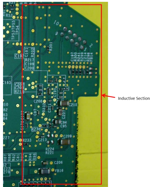
Figure 10 BSC Model 3300 – Telemetry PCA Inductive Section Bottom
