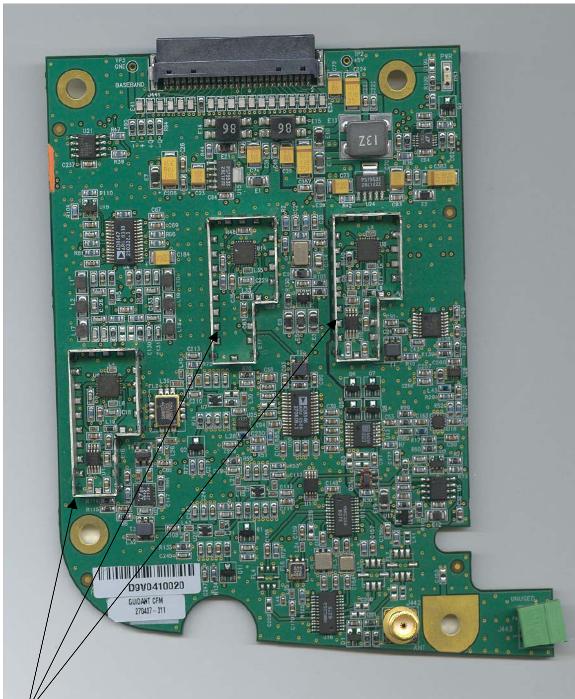
3120 Zoom Latitude Programming System 915 MHz Radio Module Top Side without Localized Shielding
