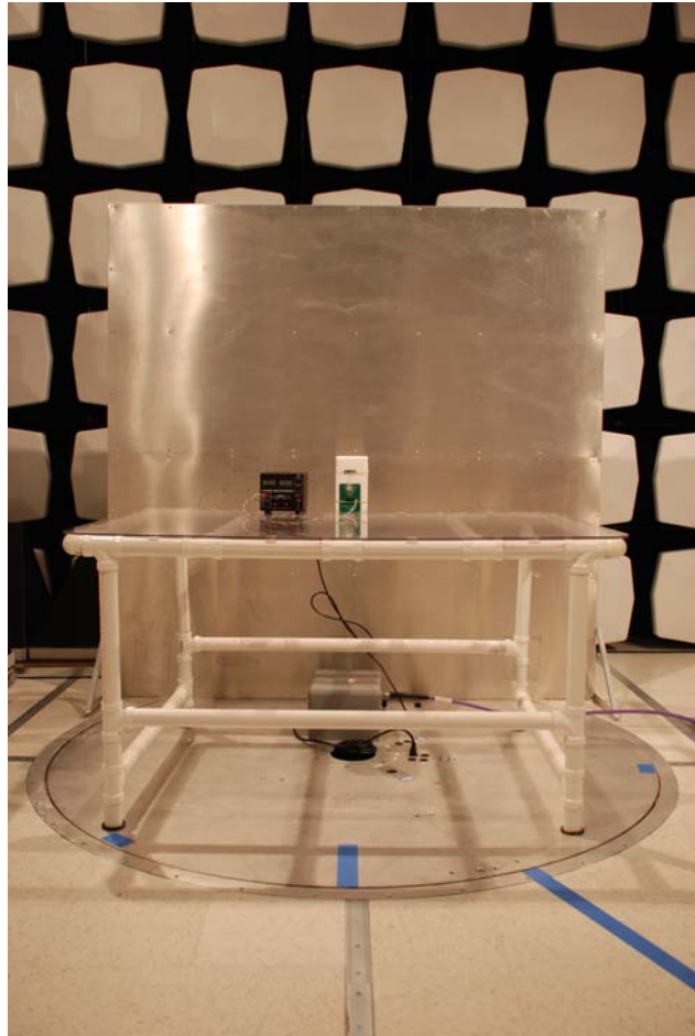
Worst-case conducted emission, front view
