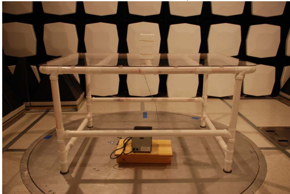
Worst-case radiated emission, rear view
