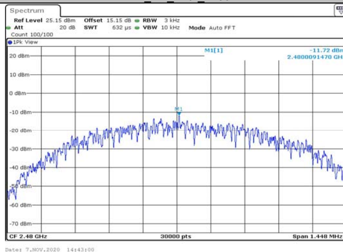
BLE_1M_Ant1_2480
