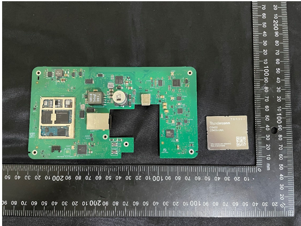
(11) EUT Photo_M202404002
