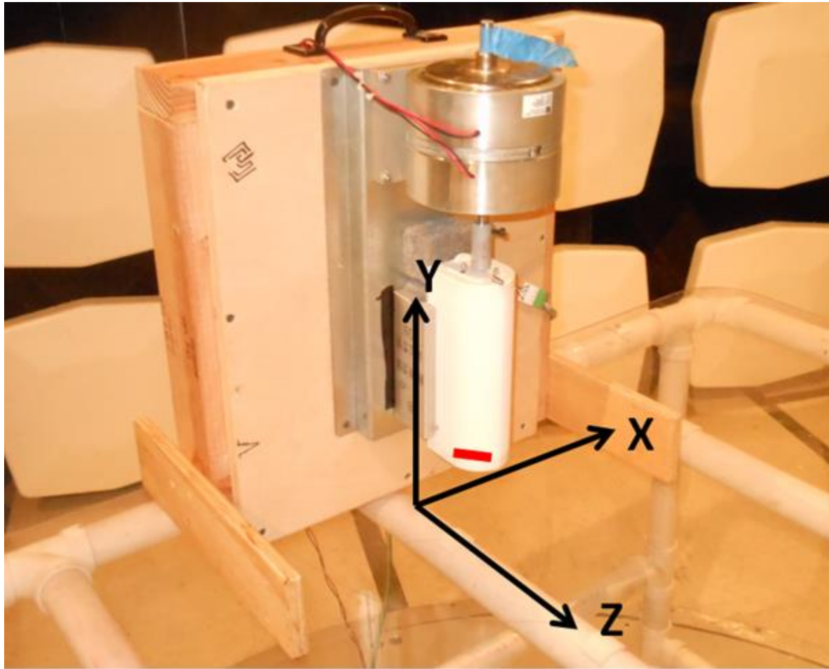
Radiated EMI
