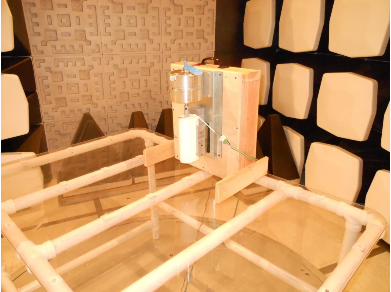
Radiated EMI
