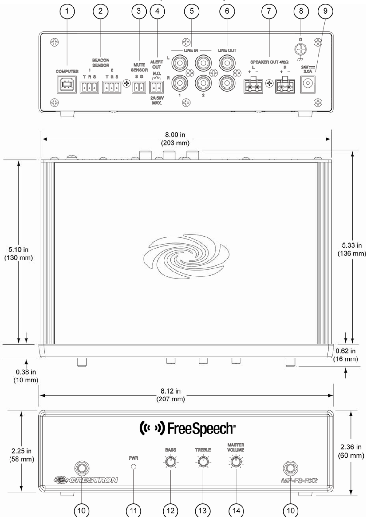
MP-FS-RX1/RX2 Overall Dimensions (MP-FS-RX2 Shown)
