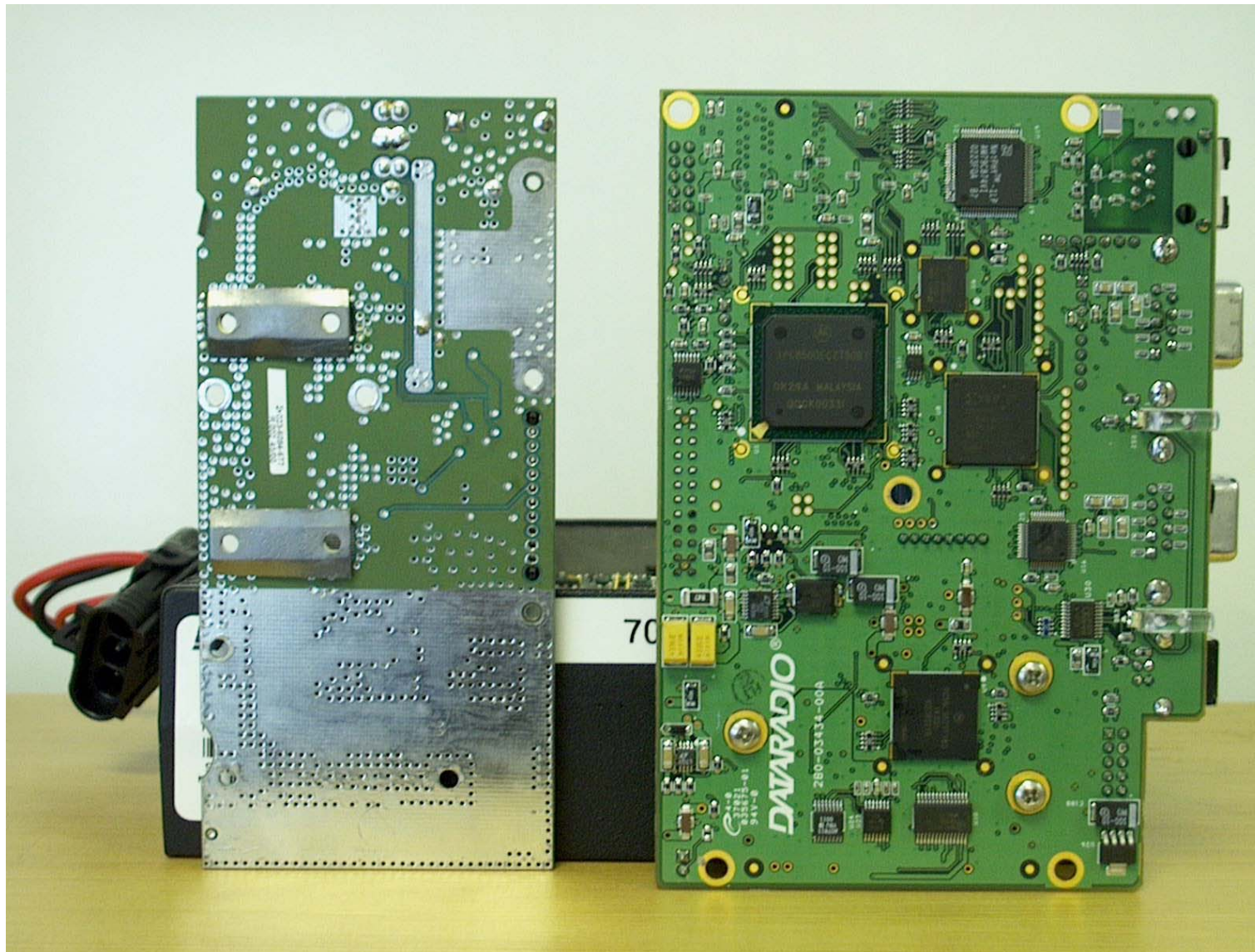
PA board (toward left) and G3 modem board (toward right) – soldering side
