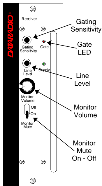
Figure 6 - Receiver module front panel
