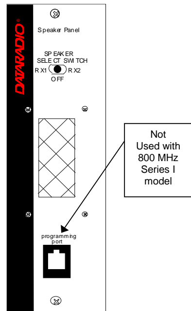
Figure 9 - Speaker panel
