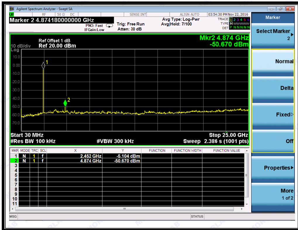
(Plot H.1: Channel = 39, 30MHz to 25GHz @ 8-DPSK)
