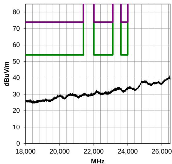
18000-26500 MHz, Run 56
