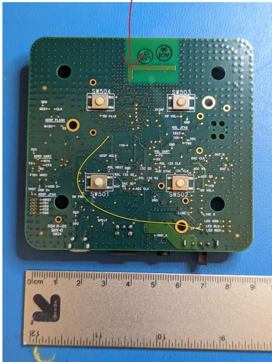
PCB board top (scale in cm above scale in inches)
