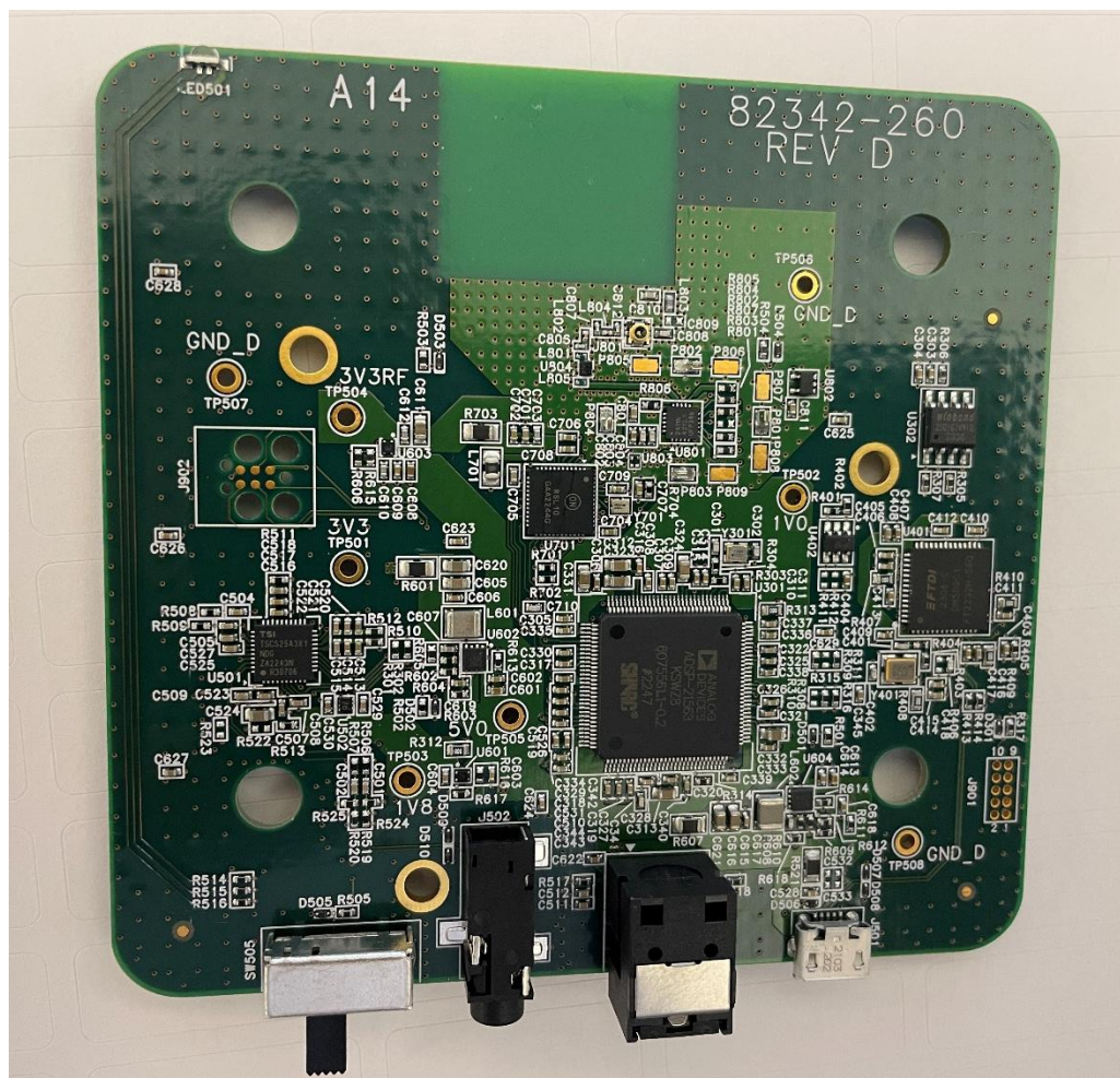
PC Board bottom side with shield over Skyworks RFX2411N RF Power Amplifier removed
