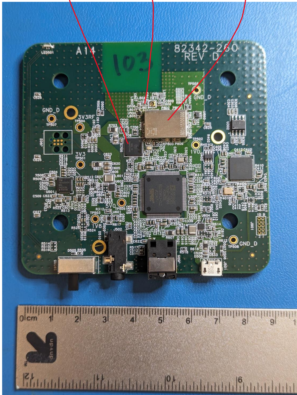
PC board bottom side (scale in cm above scale in inches)
