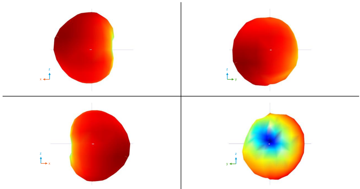
Figure 2a 3-Dimensional Antenna Pattern at 2440 MHz
