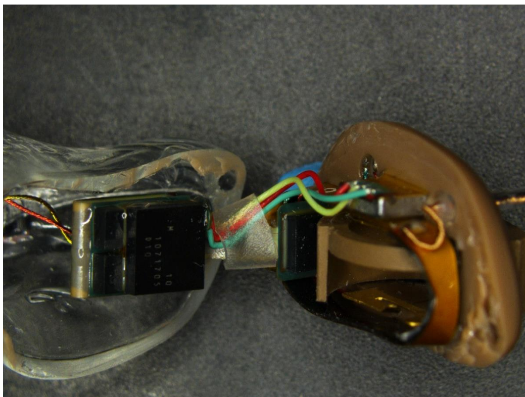
End 1 view
