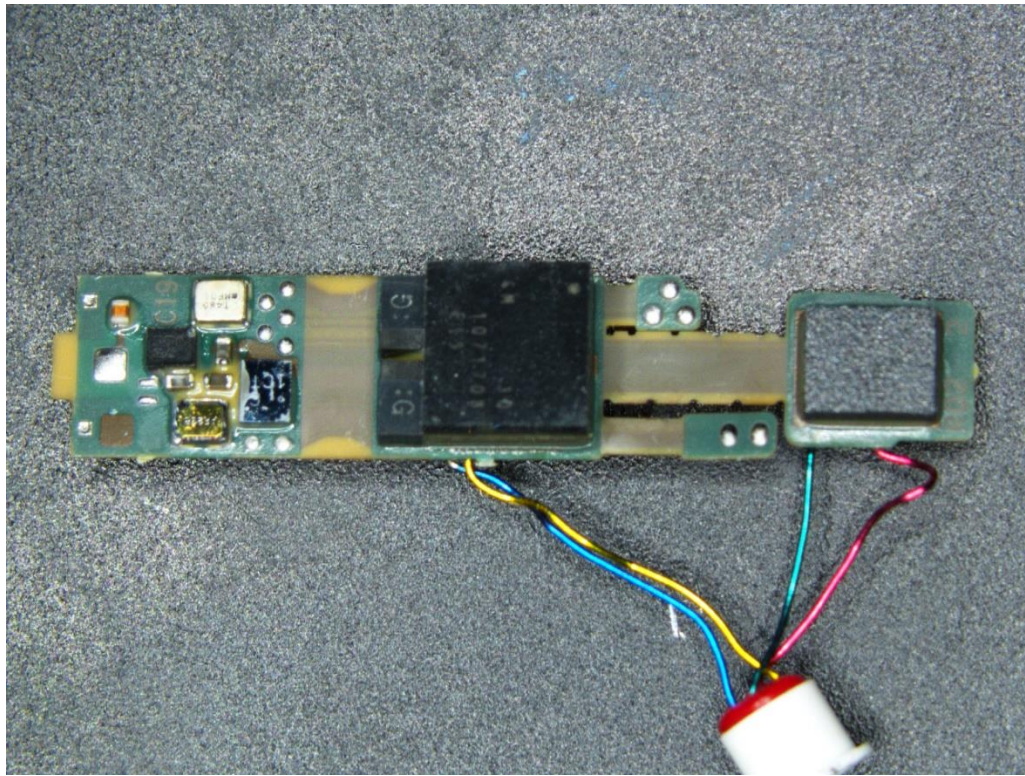
PCB front side
