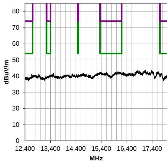
12400-18000 MHz, Run 13
