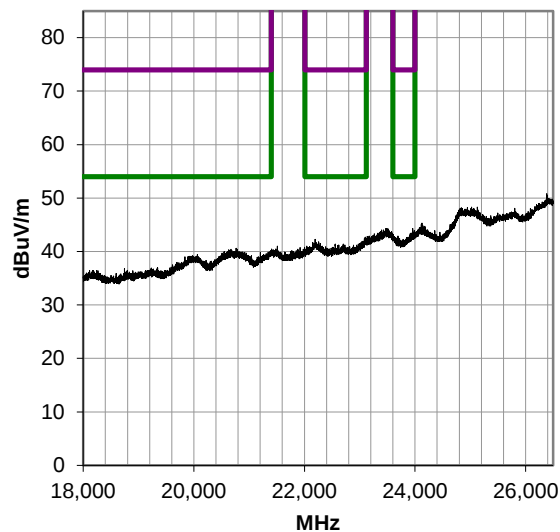
18000-26500 MHz, Run 35
