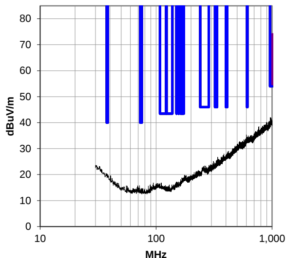
30-1000 MHz, Run 26
