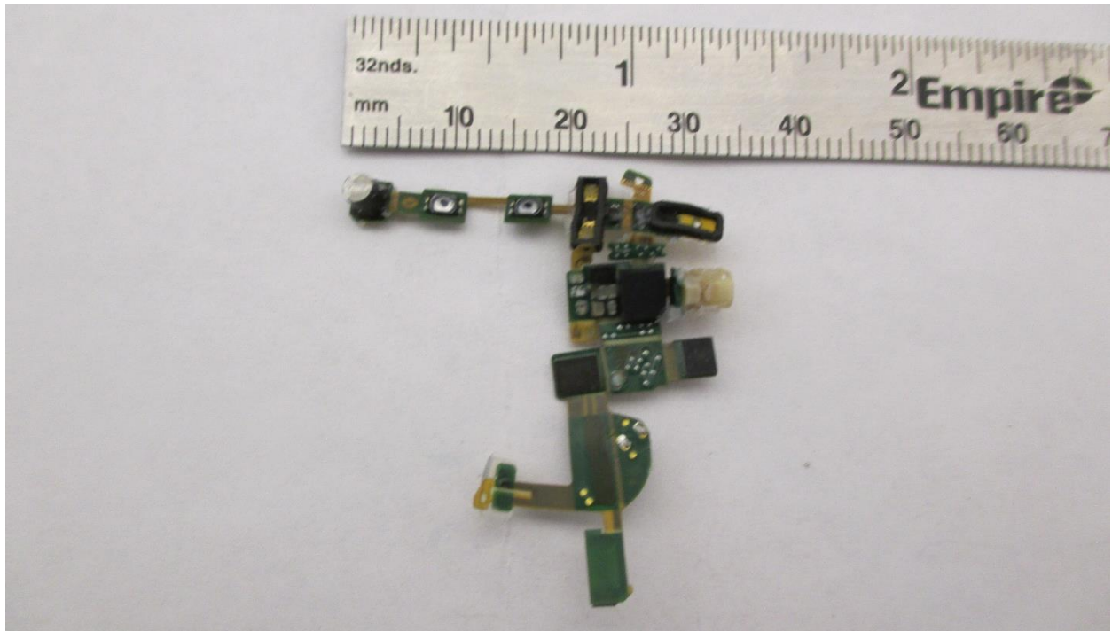
PCBA back
