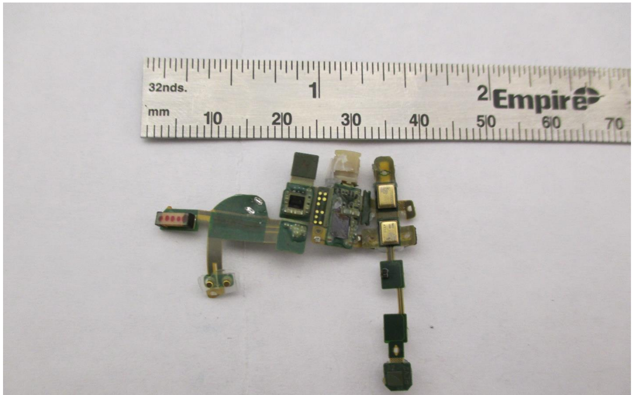
PCBA front
