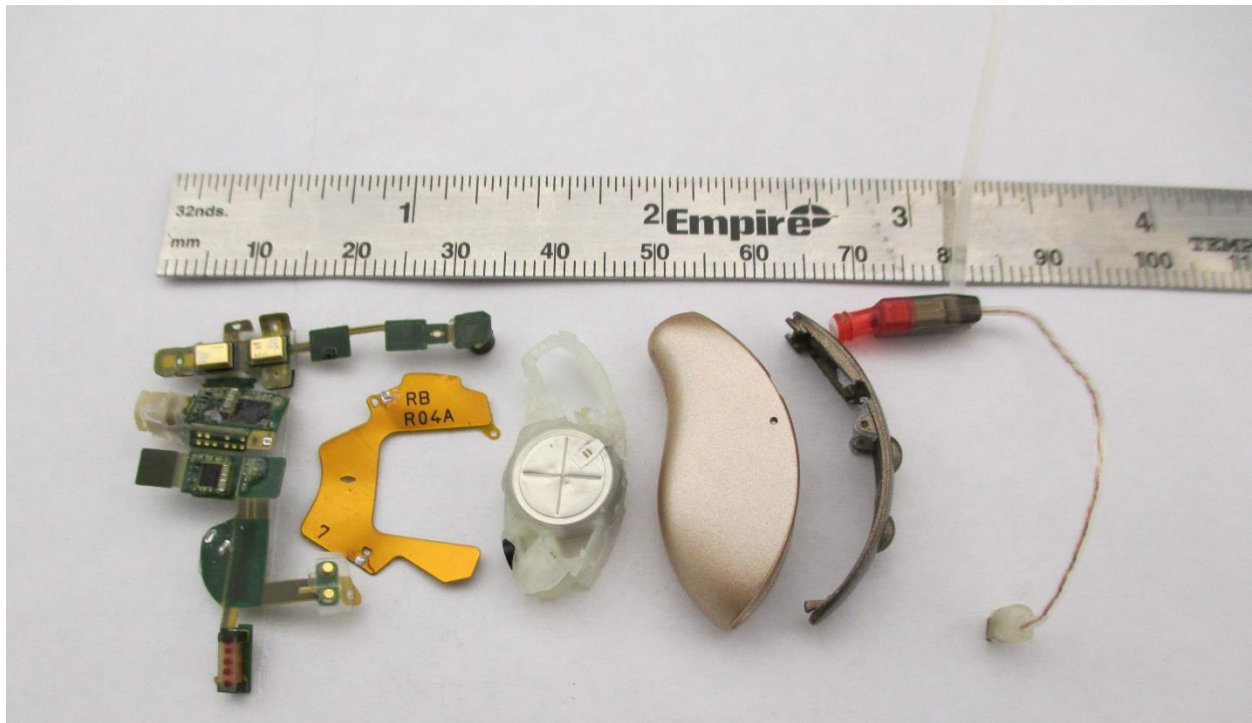
Overall assembly
