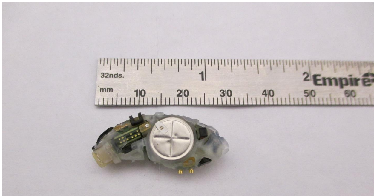
left side without antenna, showing battery case
