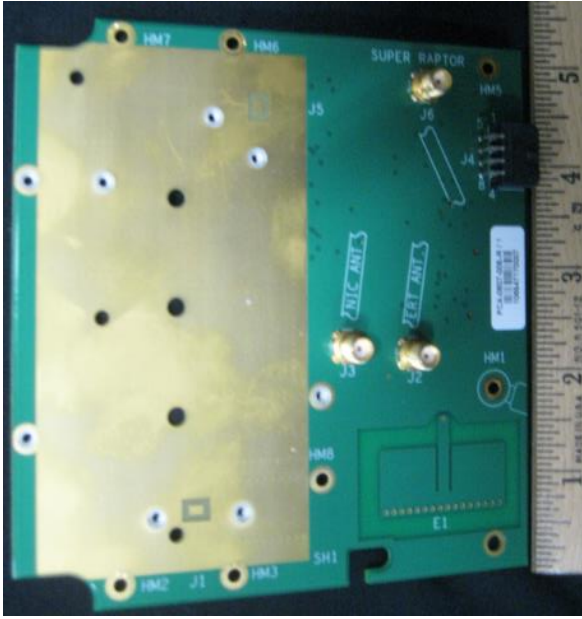
RF Switch Board - Top View
