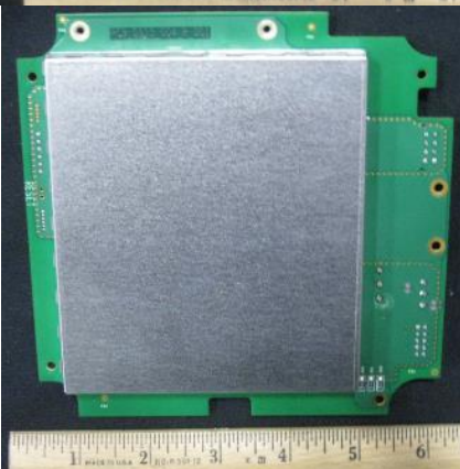
Base Board - Back View
