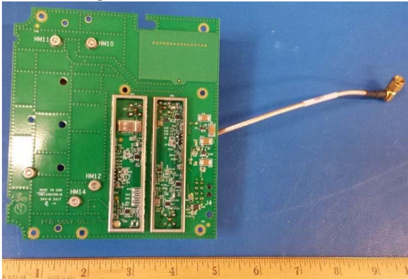
RF switching board:
