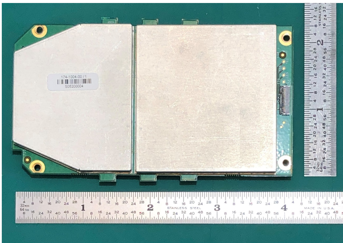
Radio board - Bottom Side w/shield (all devices)
