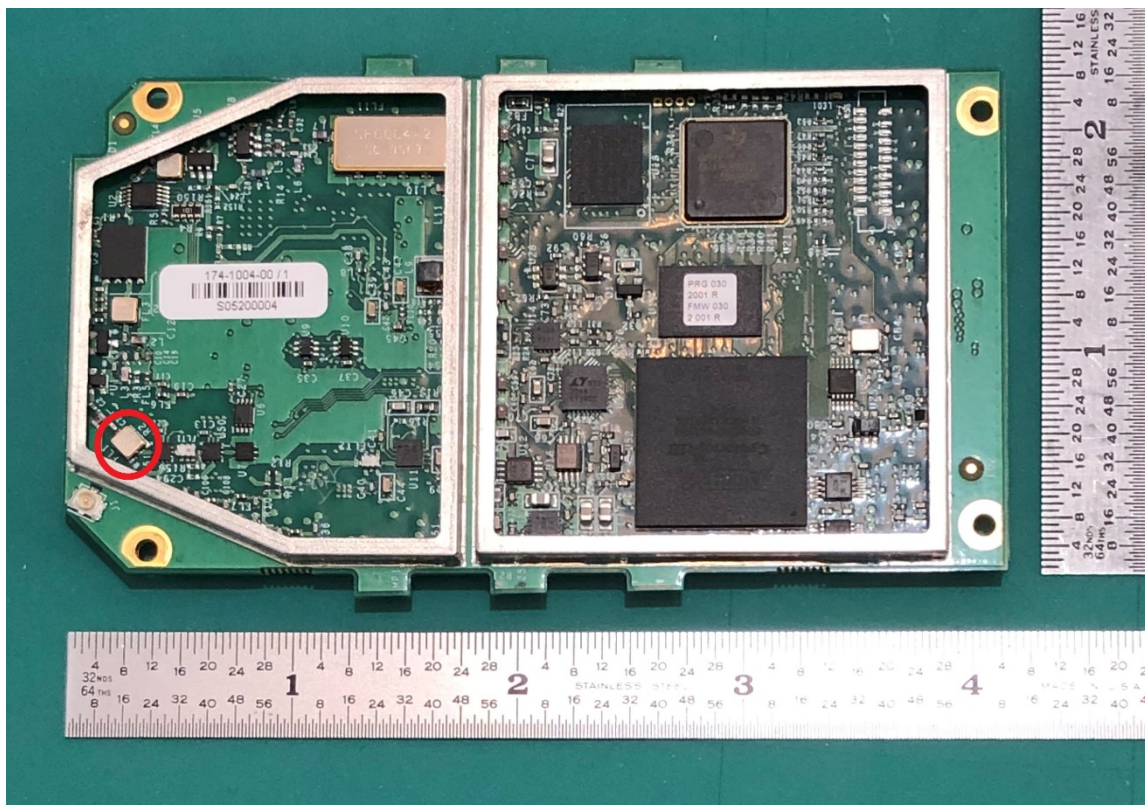
Filter FL1 (circled) not used on IMRC-EXT radio
