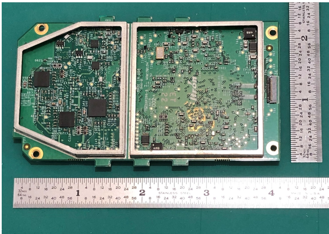
Radio board - Bottom Side w/o shield (all devices)
