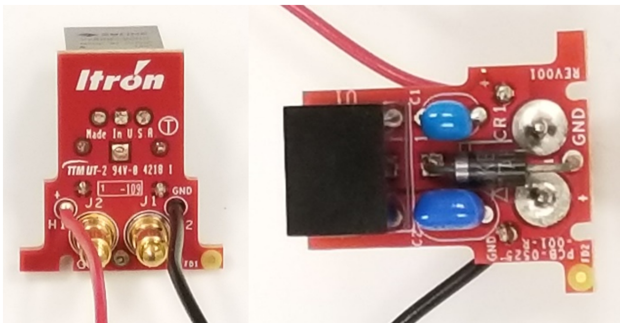
Charge Pin Board - Top and Bottom Sides (IMRC-EXT only)
