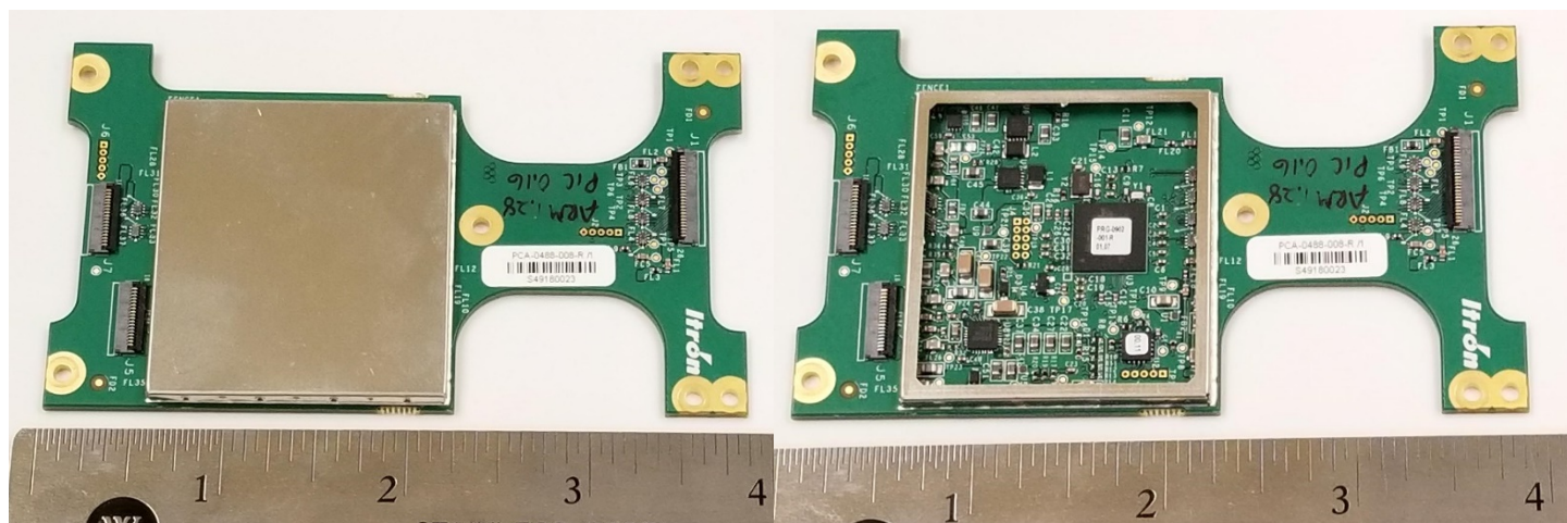
Host board (all devices)
