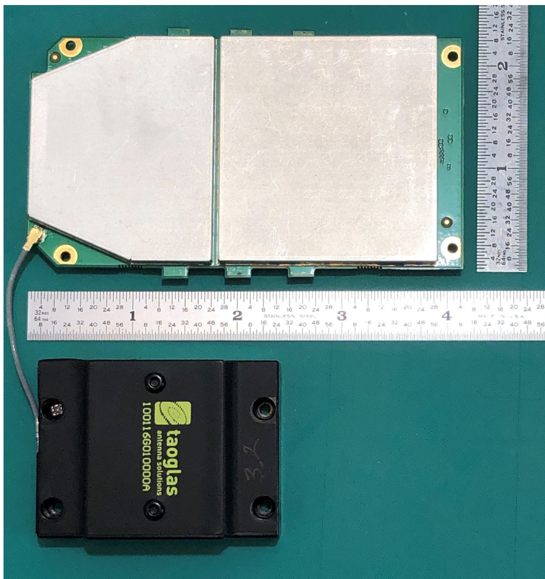
Radio board - Top Side w/shield (all devices) Taoglas internal antenna attached(IMRC-INT only)
