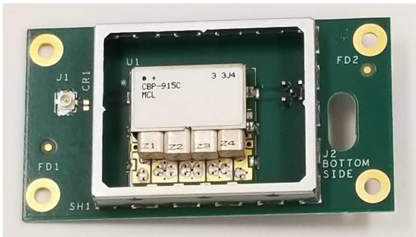
External Filter Board - Top Side, shield removed
