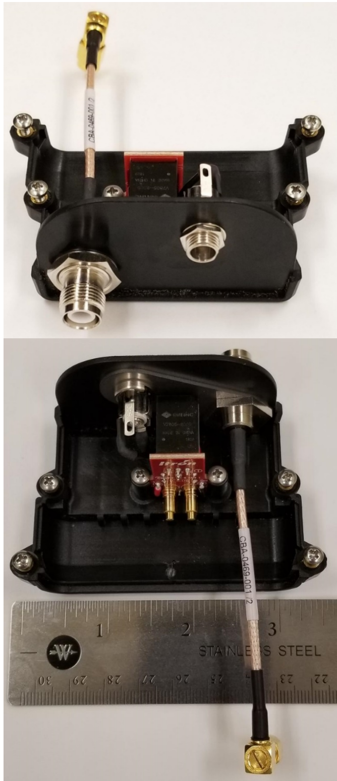
More of the base snap on feature (IMRC-EXT only)
