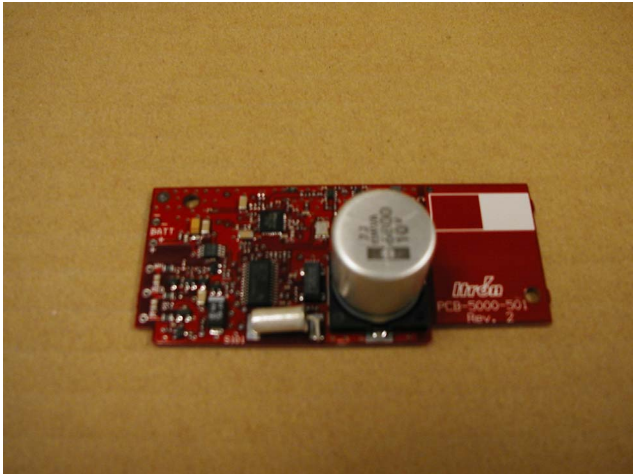
100G Remote circuit board
