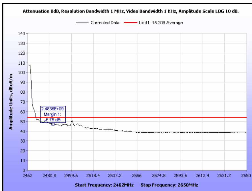
Plot 442. Radiated Restricted Band Edge, High Channel, 802.11n 5 MHz, Omni Antenna, Average
