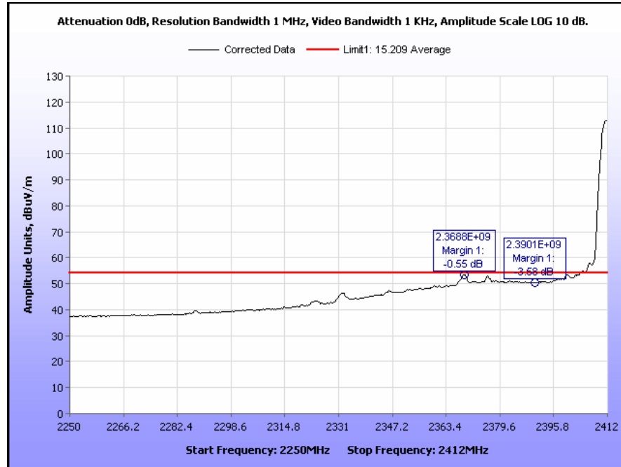
Plot 476. Radiated Restricted Band Edge, Low Channel, 802.11b 5 MHz, Parabolic Antenna, Average
