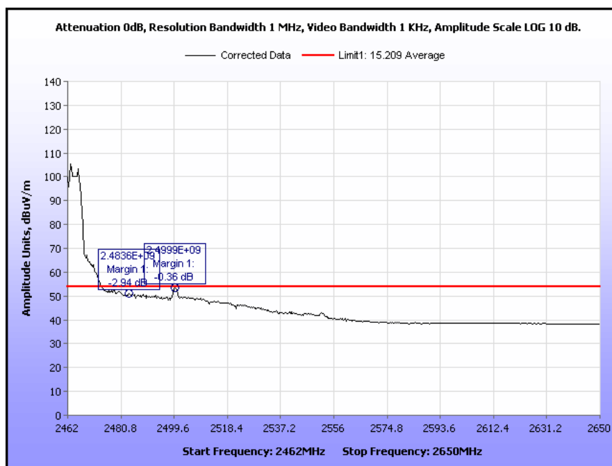
Plot 538. Radiated Restricted Band Edge, High Channel, 802.11g 10 MHz, Yagi Antenna, Average
