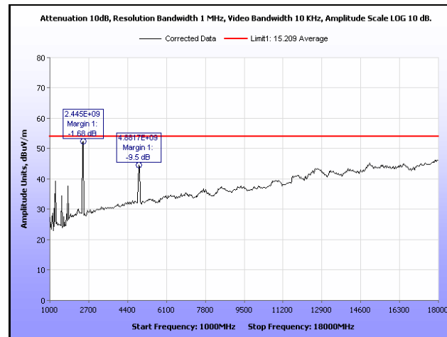
Plot 427. Radiated Spurious Emissions, Mid Channel, 802.11n 40 MHz, Yagi Antenna, 1 GHz – 18 GHz, Average
