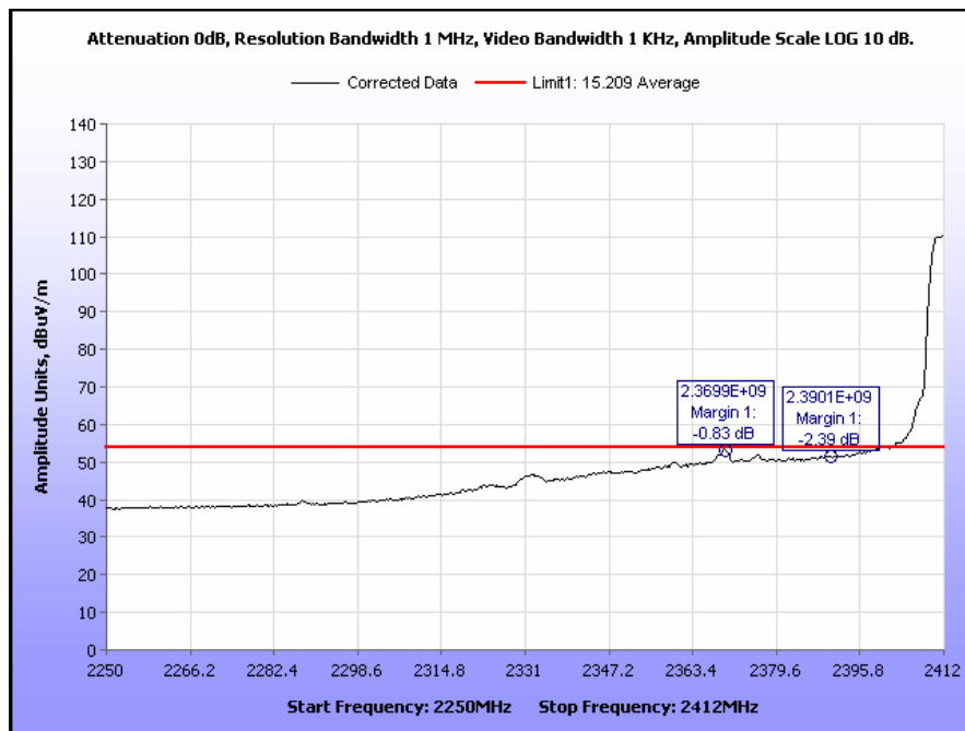
Plot 524. Radiated Restricted Band Edge, Low Channel, 802.11g 5 MHz, Yagi Antenna, Average
