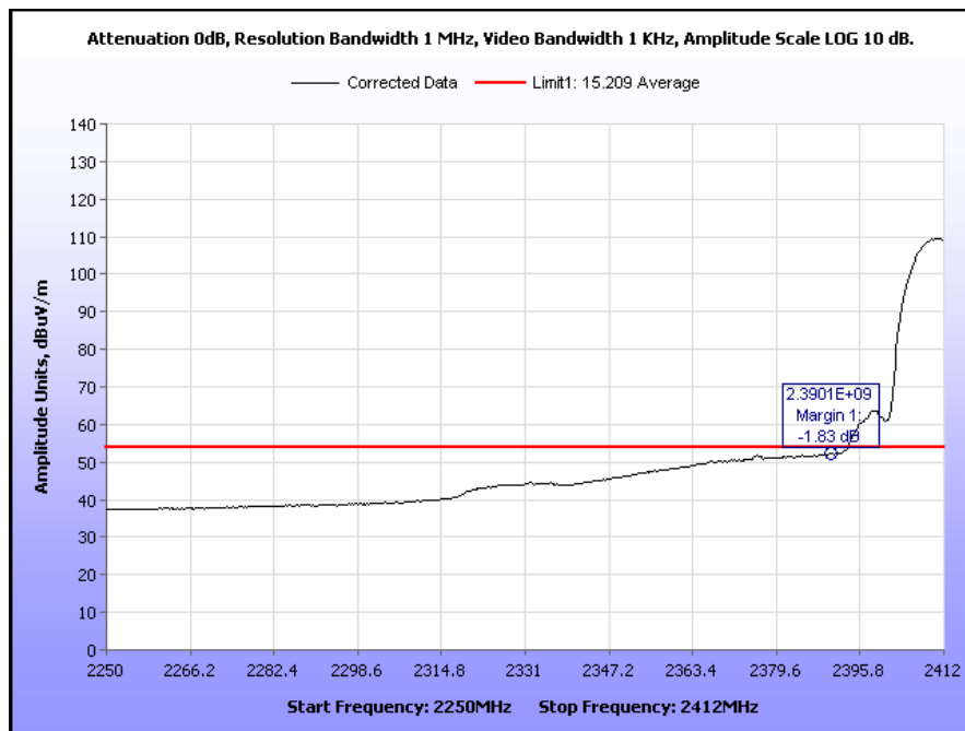
Plot 456. Radiated Restricted Band Edge, Low Channel, 802.11b 20 MHz, Omni Antenna, Average
