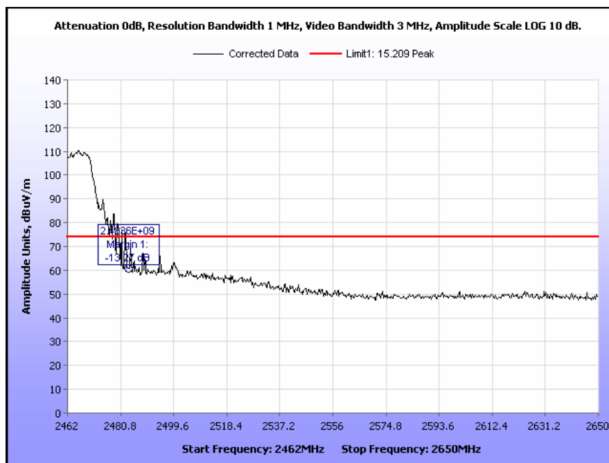
Plot 551. Radiated Restricted Band Edge, High Channel, 802.11g 20 MHz, Yagi Antenna, Peak
