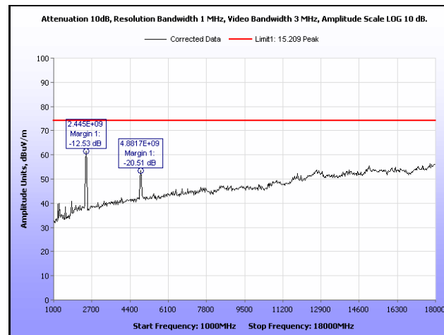
Plot 428. Radiated Spurious Emissions, Mid Channel, 802.11n 40 MHz, Yagi Antenna, 1 GHz – 18 GHz, Peak
