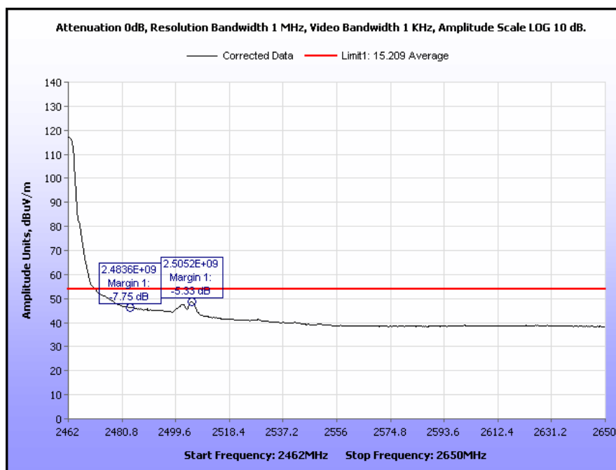
Plot 434. Radiated Restricted Band Edge, High Channel, 802.11b 5 MHz, Omni Antenna, Average
