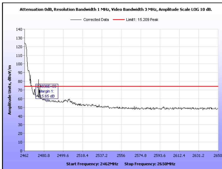
Plot 435. Radiated Restricted Band Edge, High Channel, 802.11b 5 MHz, Omni Antenna, Peak
