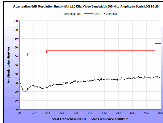
Plot 426. Radiated Spurious Emissions, Mid Channel, 802.11n 40 MHz, Yagi Antenna, 30 MHz – 1 GHz
