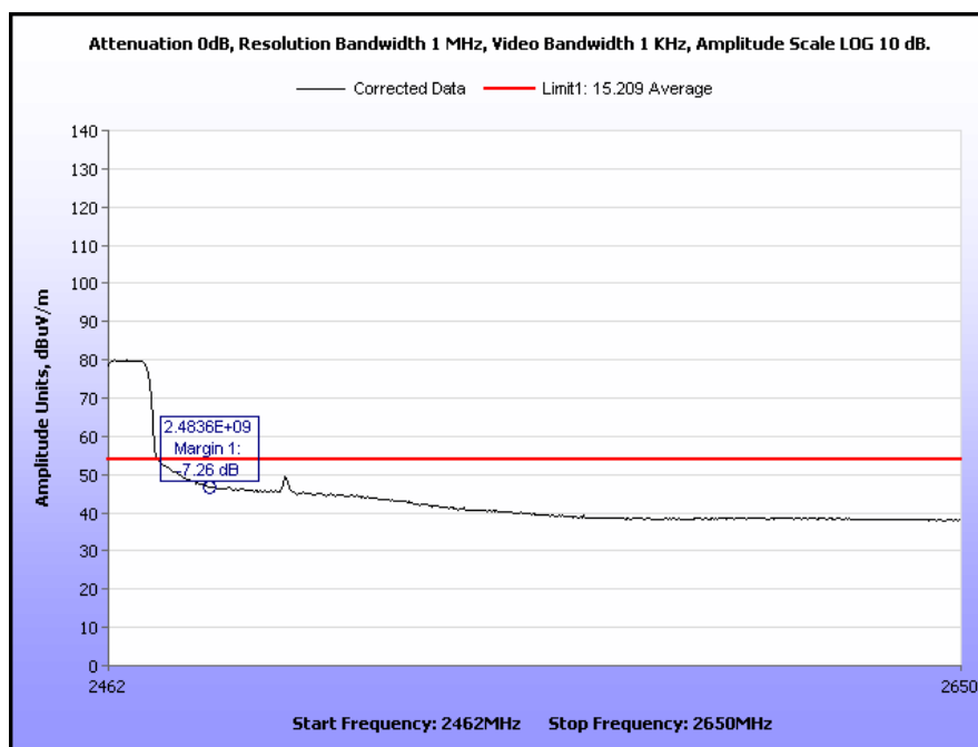
Plot 550. Radiated Restricted Band Edge, High Channel, 802.11g 20 MHz, Yagi Antenna, Average
