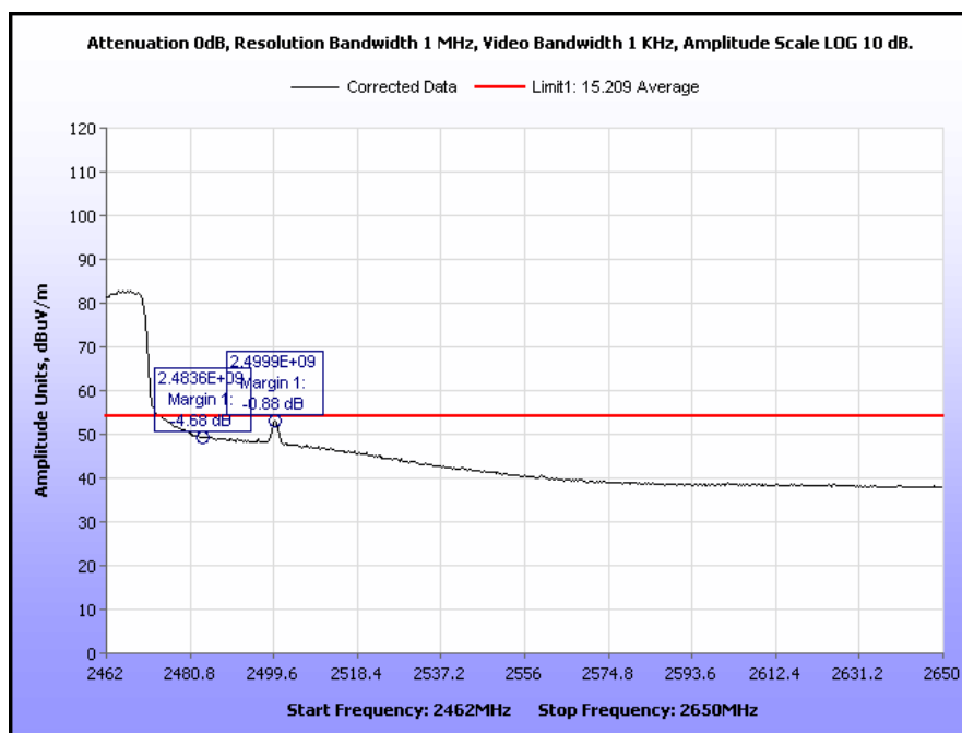
Plot 506. Radiated Restricted Band Edge, High Channel, 802.11g 20 MHz, Parabolic Antenna, Average
