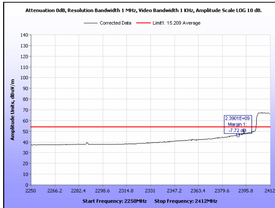
Plot 472. Radiated Restricted Band Edge, Low Channel, 802.11n 40 MHz, Omni Antenna, Average
