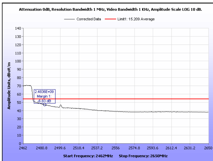
Plot 558. Radiated Restricted Band Edge, High Channel, 802.11g 40 MHz, Yagi Antenna, Average
