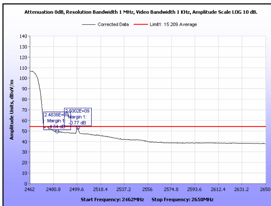
Plot 546. Radiated Restricted Band Edge, High Channel, 802.11b 20 MHz, Yagi Antenna, Average
