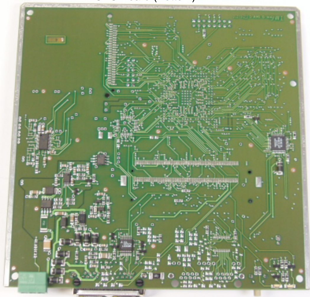
CPU Board (Bottom)
