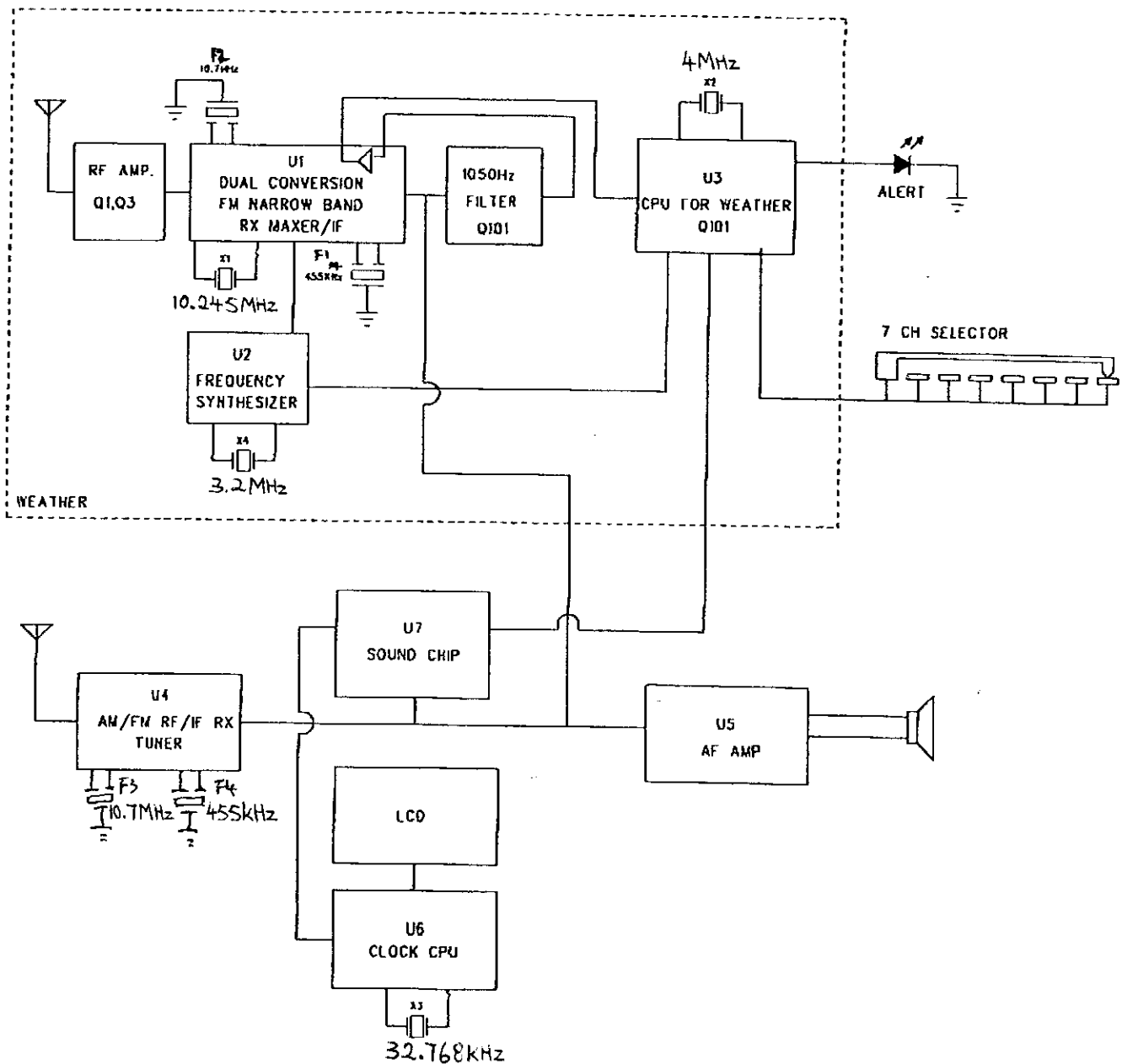
T-463 BLOCK DIAGRAM
