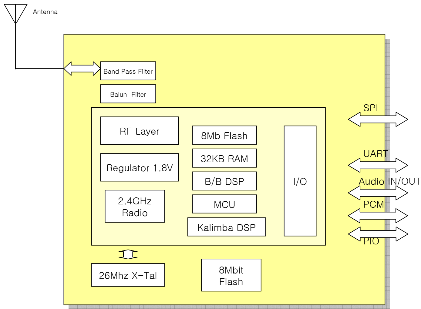
MB0302MM Block Diagram
