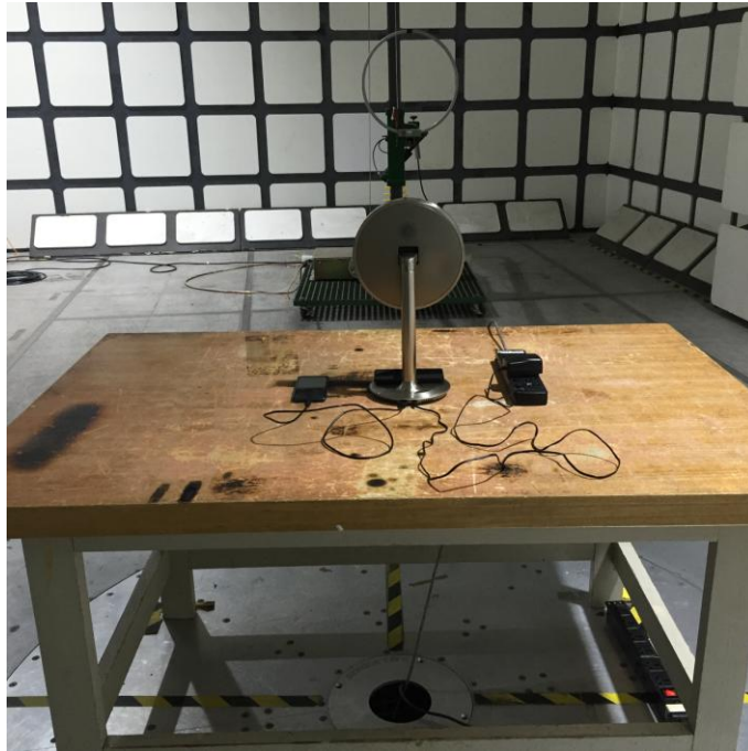
Radiated Emissions View (9 kHz ~ 30 MHz)
