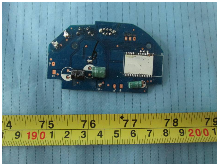
EUT – Main Board Bottom 1 with Sub-board off View
