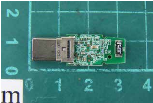
Dongle Antenna Location
