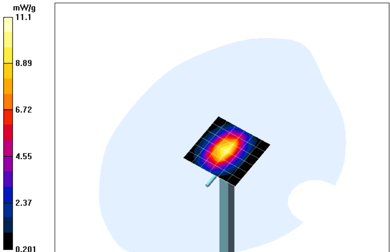
Fig. 10: Validation measurement 1900 MHz Head (April 03, 2007), coarse grid. Ambient Temperature: 22.4° C, Liquid Temperature: 21.2° C.
