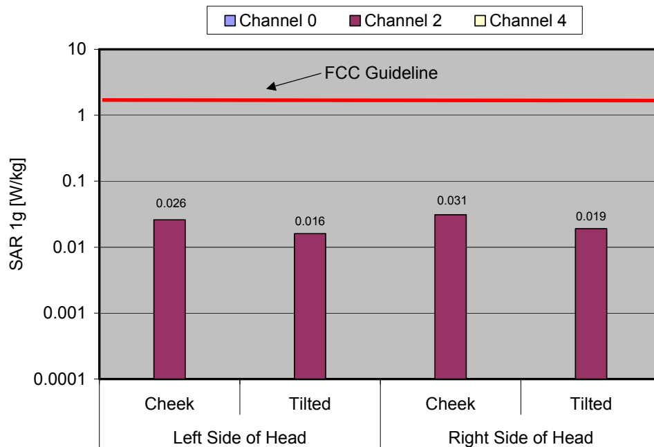
Fig. 8: The measured head phantom SAR values for the RTX Dualphone 3088.1 for the US DECT standard in comparison to the FCC exposure limit.
