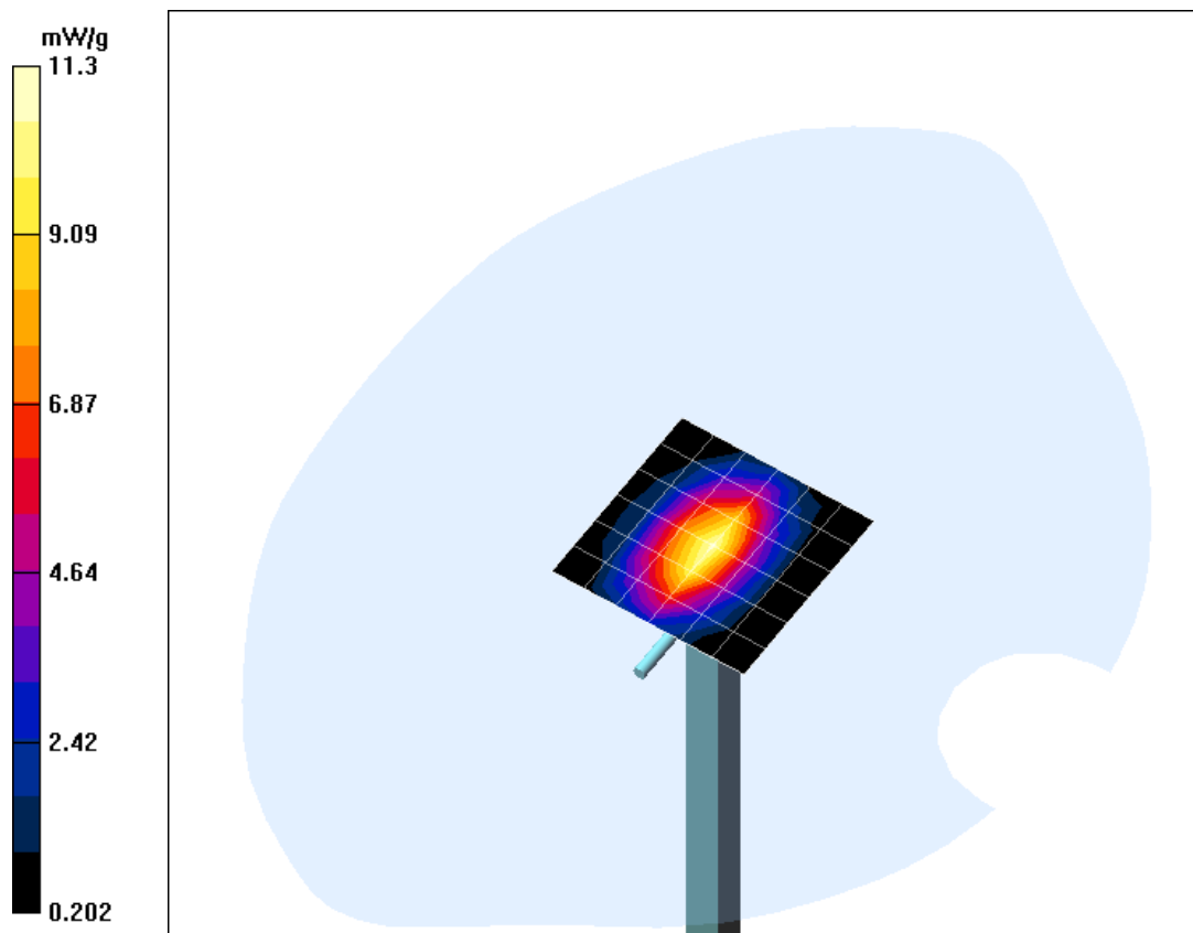
Fig. 11: Validation measurement 1900 MHz body (April 03, 2007), coarse grid. Ambient Temperature: 22.6° C, Liquid Temperature: 21.3° C.
