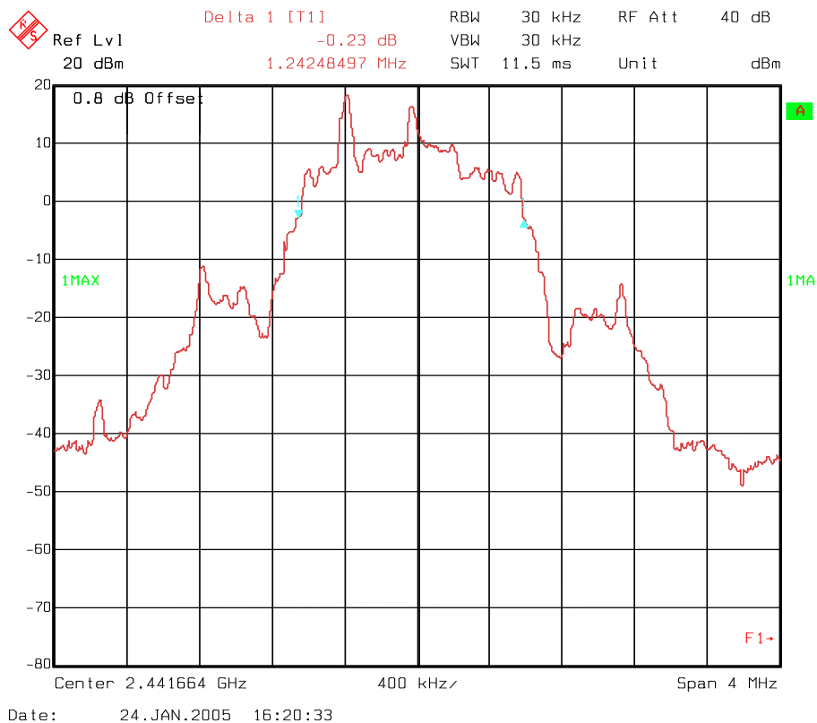
20 dB Bandwidth
