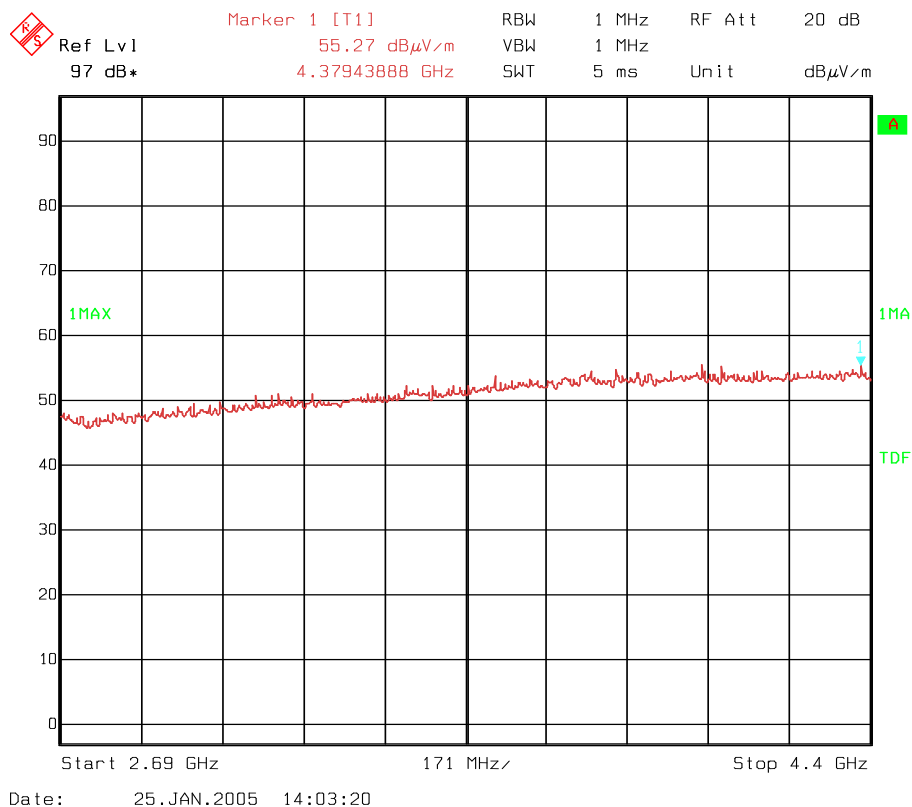
RF radiated emissions 2.69-4.4 GHz channel 0
