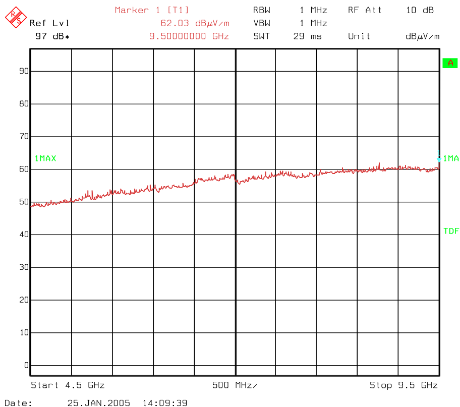
RF radiated emissions 4.5-9.5 GHz channel 0
