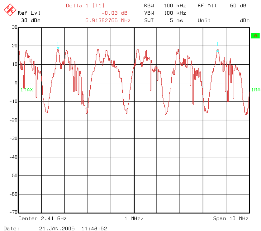
Channel separation
