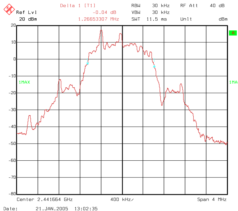
20 dB Bandwidth
