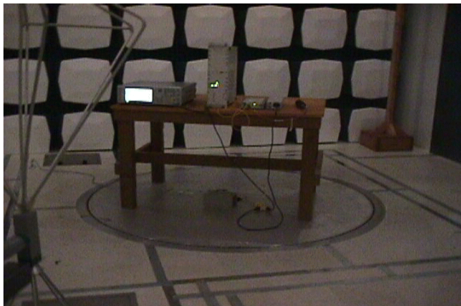
Photograph of Radiated Emissions Test Configuration
