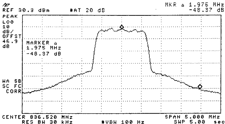
Figure C1.8 IS-95/97-A Mask 48.37 +16 64.37 dBc
