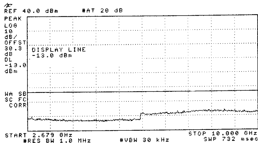
Figure C1.5 FORWARD FCC limit: -13 dBm
