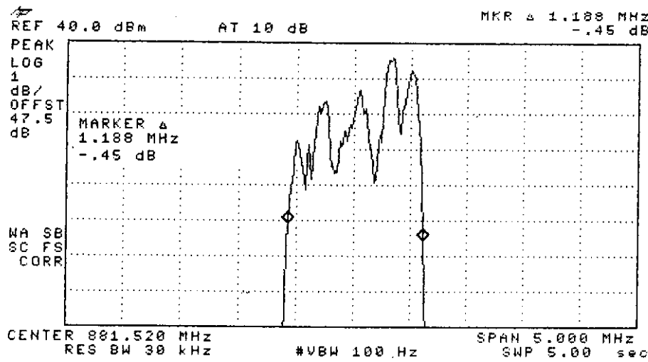
Figure C2.1 Repeater CDMA FORWARD Output Bandwidth
