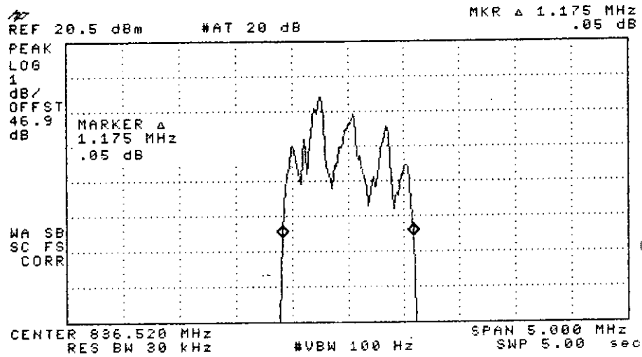
Figure C2.3 Repeater CDMA REVERSE Output Bandwidth
