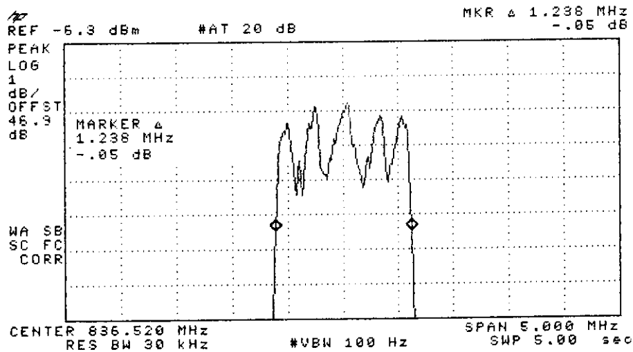
Figure C2.4 Test Source CDMA Output Bandwidth
