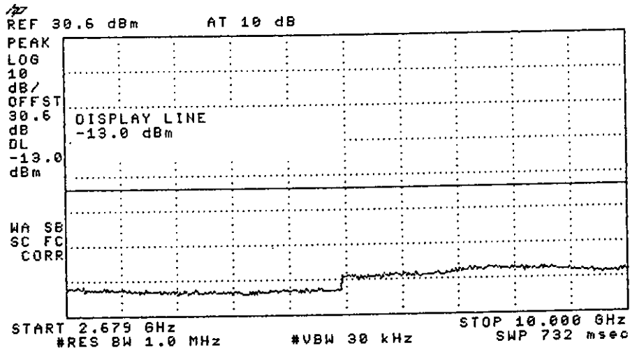
Figure C3.4 REVERSE FCC limit: -13 dBm
