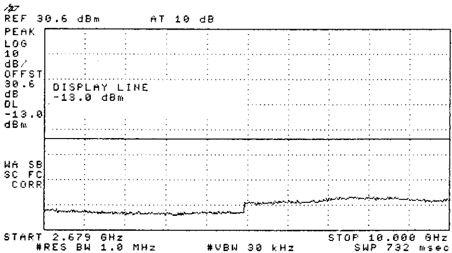
Figure C1.10 REVERSE FCC limit: -13 dBm
