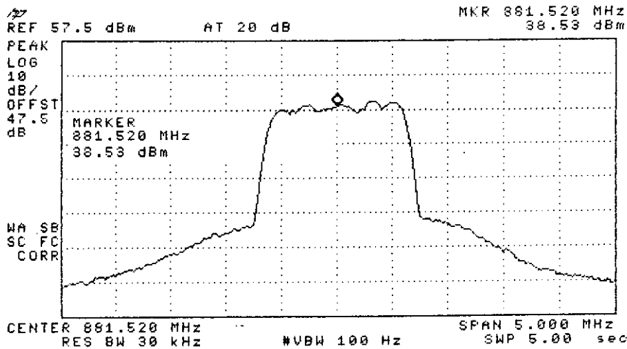
Figure C1.1 Forward Rated Output Power
