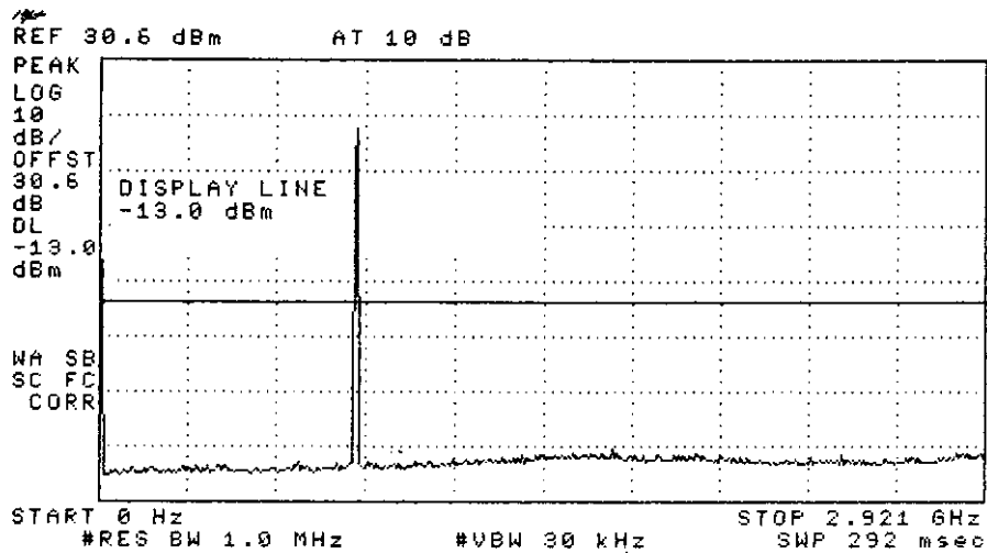
Figure C1.9 REVERSE FCC limit: -13 dBm
