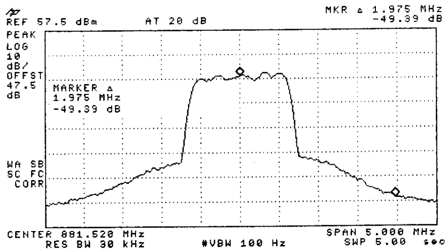
Figure C1.3 IS-95/97-A Mask 49.39 +16 65.39 dBc
