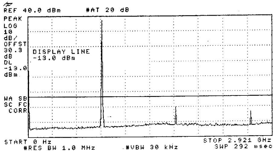
Figure C1.4 FORWARD FCC limit: -13 dBm
