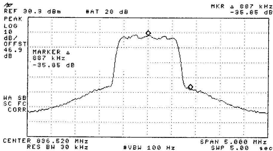
Figure C1.7 IS-95/97-A Mask 35.85 +16 51.85 dBc
