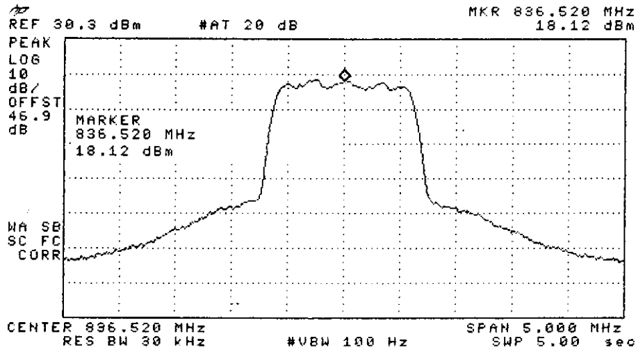
Figure C1.6 Reverse Rated Output Power
