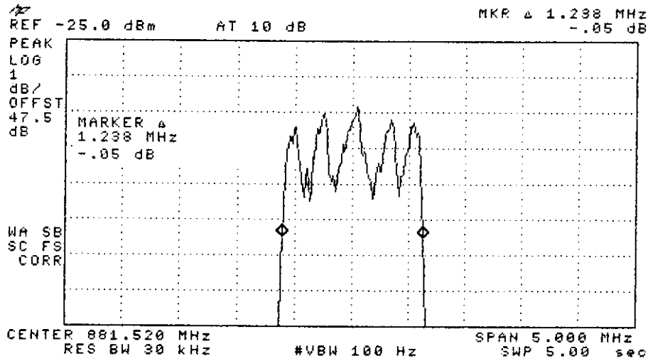
Figure C2.2 Test Source CDMA Output Bandwidth
