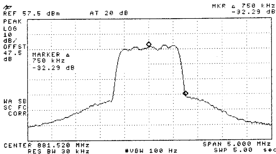
Figure C1.2 IS-95/97-A Mask 32.29 +16 48.29 dBc
