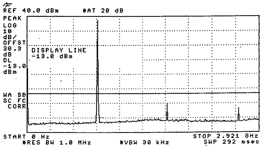
Figure C3.1 FORWARD FCC limit: -13 dBm
