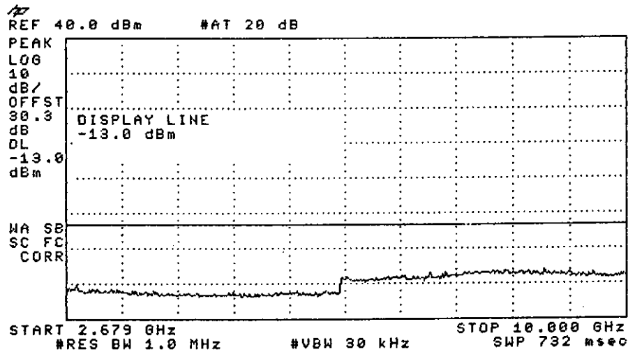
Figure C3.2 FORWARD FCC limit: -13 dBm
