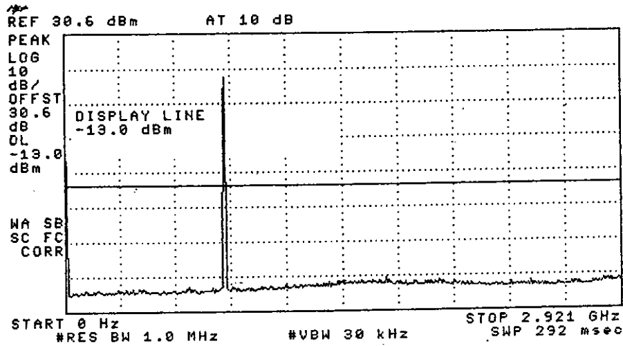
Figure C3.3 REVERSE FCC limit: -13 dBm
