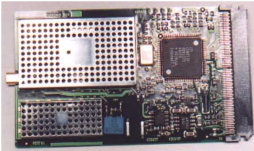
PC Card with Shields (Close Up FRONT)
