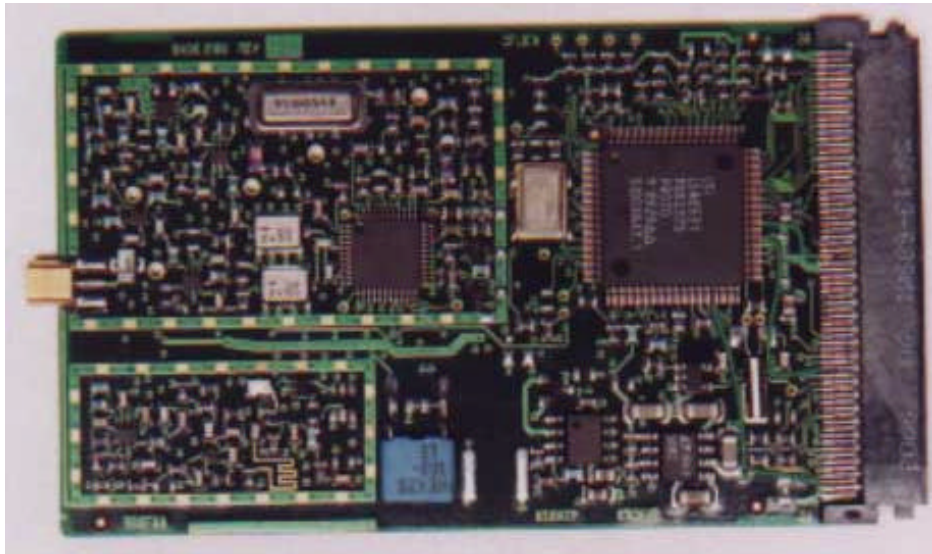
PC Card without Shields (Close Up FRONT)
