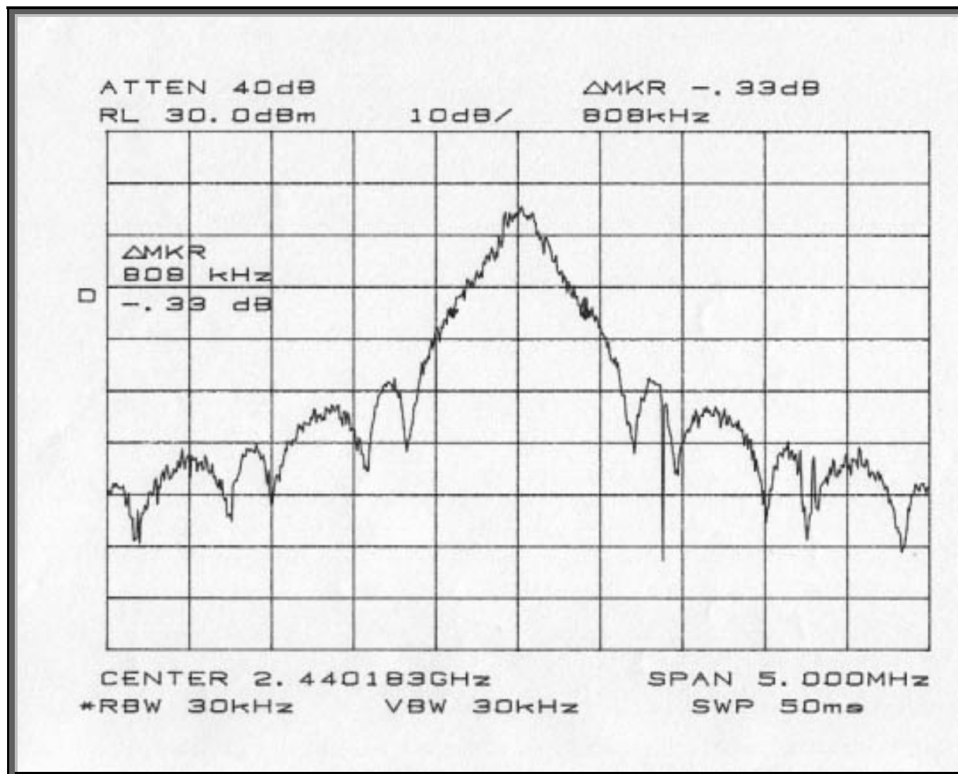
20dB Bandwidth Channel 39
