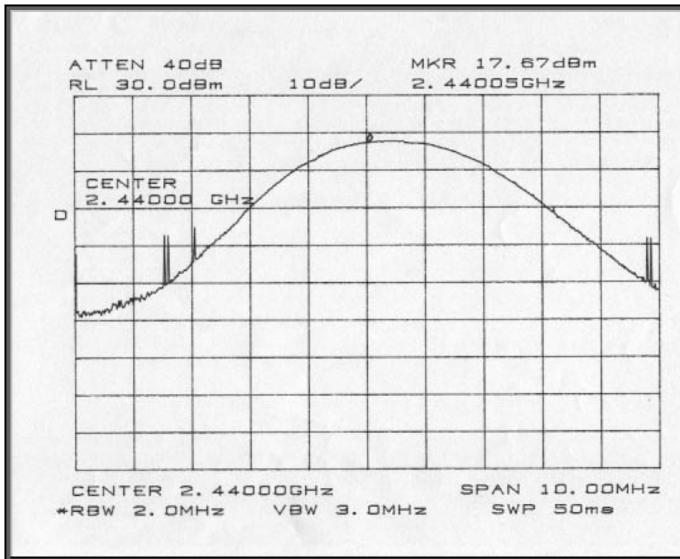
Power Out Channel 39
