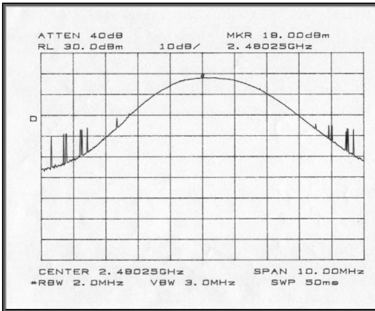
Power Out Channel 79
