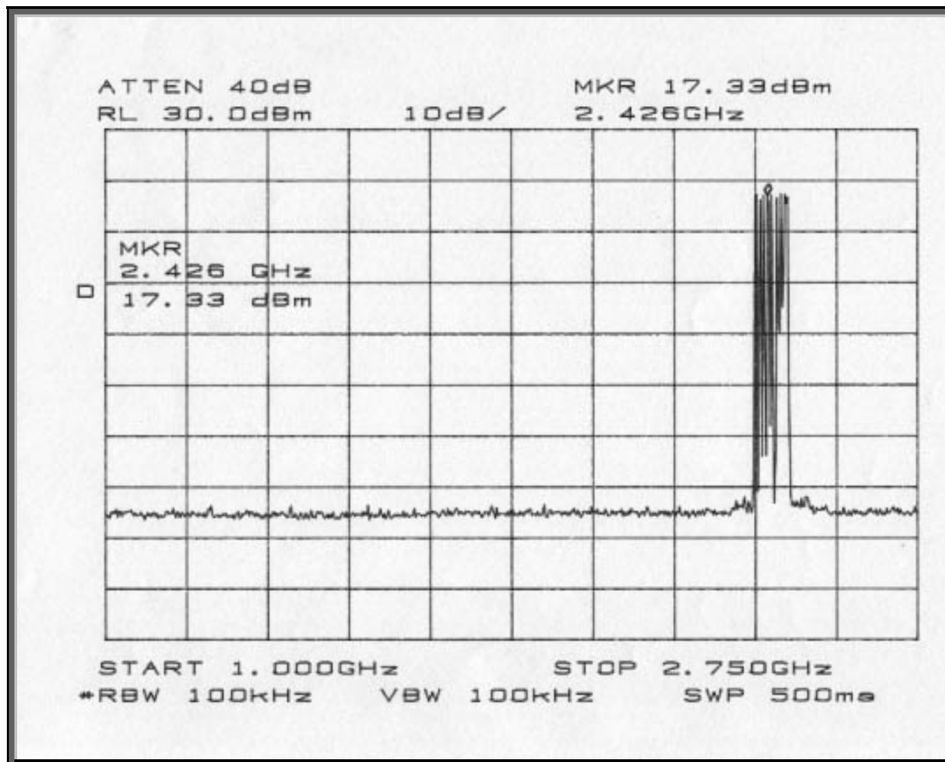
Out of Band (2)
