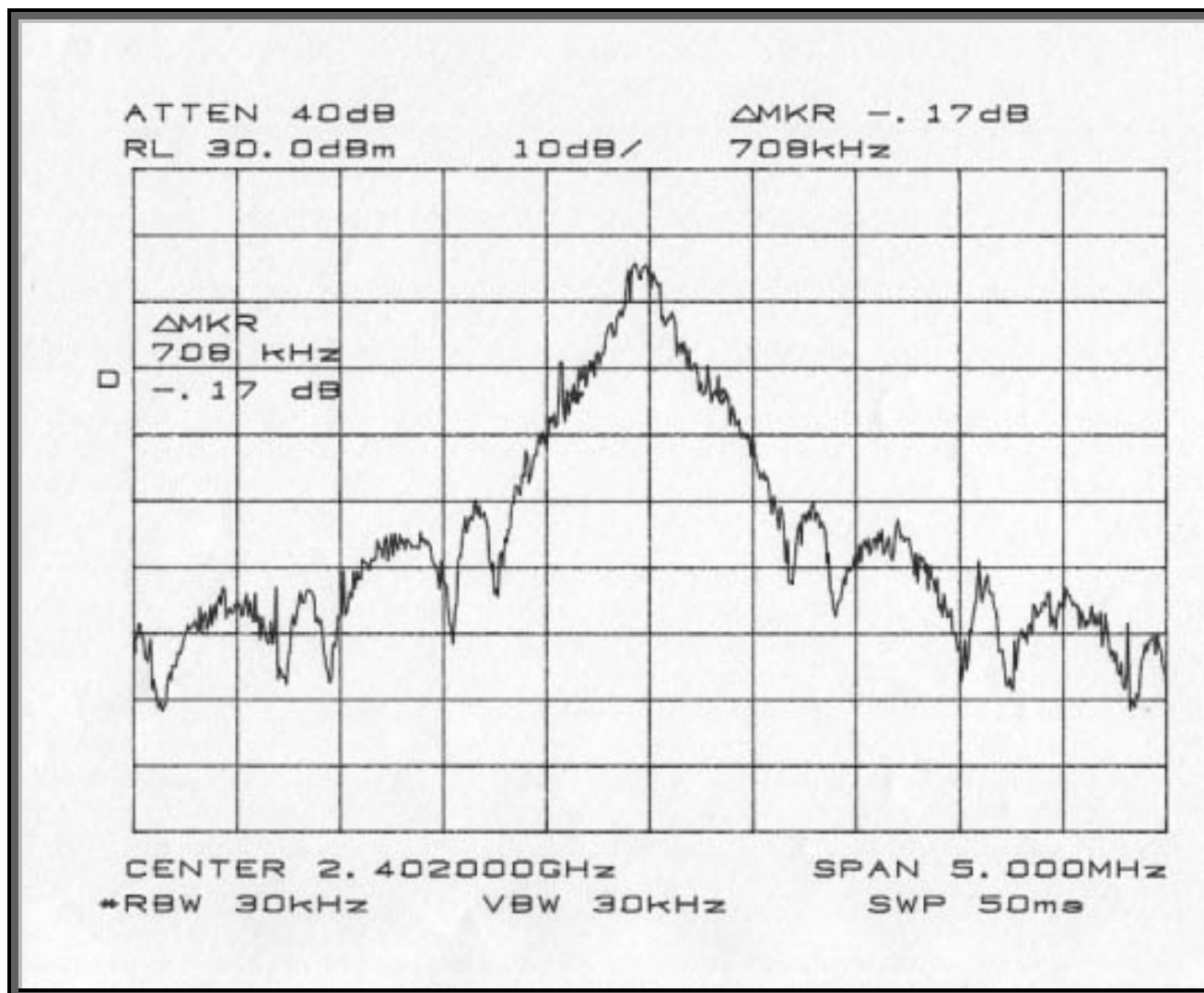
20dB Bandwidth Channel 1
