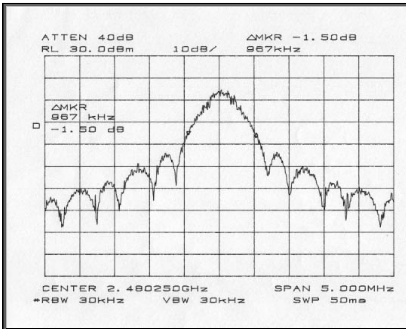
20dB Bandwidth Channel 79
