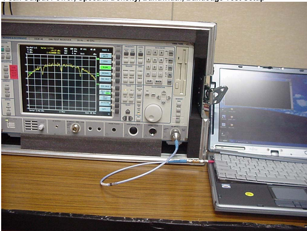
Peak Output Power, Spectral Density, Bandwidth, Bandedge Test Setup
