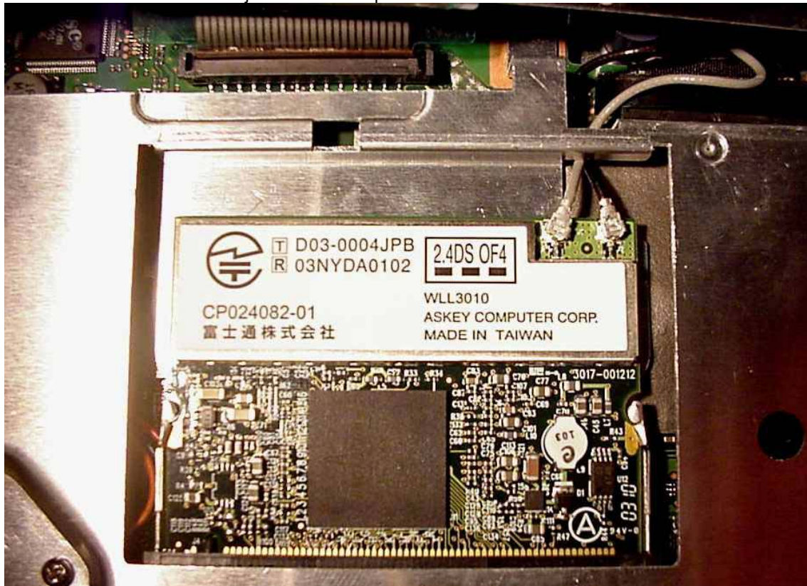
WLL3010-MACE inside the Fujitsu Tablet Computer
